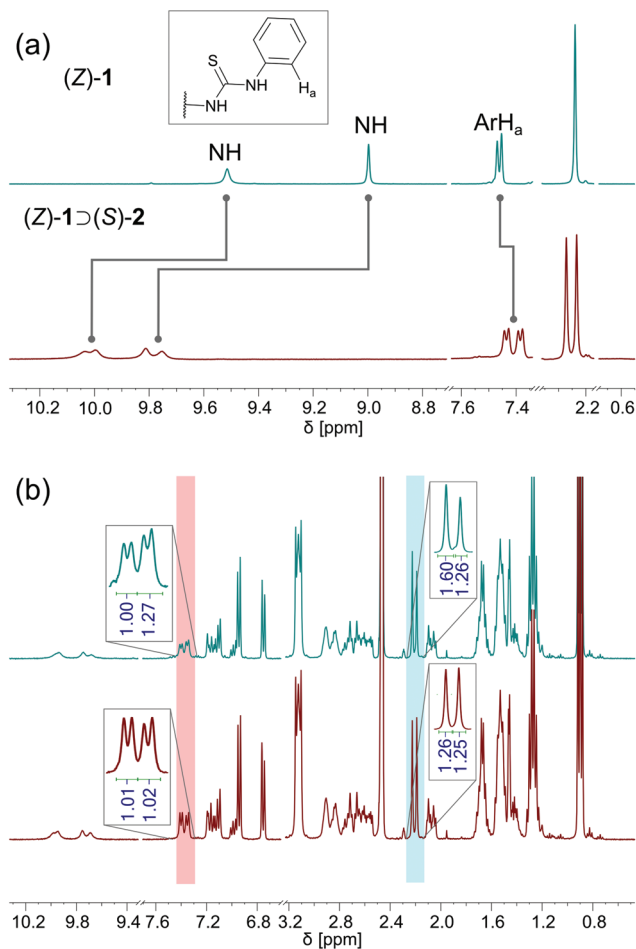
Fig. 2 (a) ^1\text{H} NMR of (Z)-1 (5 mM in DMSO- d_6 /0.5% \text{H}_2\text{O} ) before and after addition of 2 equivalents [\text{Bu}_4\text{N}]^+[(\text{S})\text{-}2]^- ; (b) ^1\text{H} NMR changes of (Z)-1 in the presence of [\text{Bu}_4\text{N}]^+[(\text{S})\text{-}2]^- freshly prepared (bottom) and after 3 days (top).
