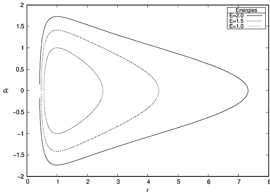
FIG. 3. The trajectories of a particle of mass m = 1 and l = 1 in d = 3 . The plots are in the phase space of the radial coordinate, (r, p_r) , for three different values of the energy, E = 1, 1.5 , and 2 . As discussed in the text, this illustrates the inescapable bounded nature of the orbits of massive particles in d = 3 Newtonian gravity.
