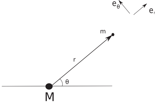
FIG. 1. In the text we consider the effective potential V_{\text{eff}} of a configuration with a very large mass M interacting with a pointlike mass m ( M \gg m ).
