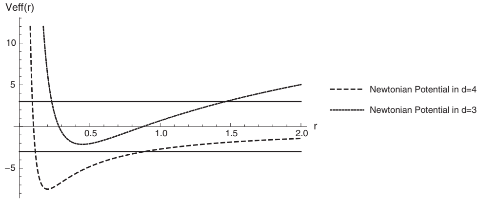
FIG. 2. The Newtonian gravitational effective potential in d = 3 (short dashes) and in d = 4 (long dashes). The horizontal continuous lines, that refer to arbitrary values of the total energy E , help visualize that, for any value of the allowed energies E , the orbits in d = 3 are always bounded; i.e., the value of r can never exceed a value fixed by the intersection of V_{\text{eff}} and the given horizontal line (here, roughly given by r \simeq 1.5 for E = +3 ).
