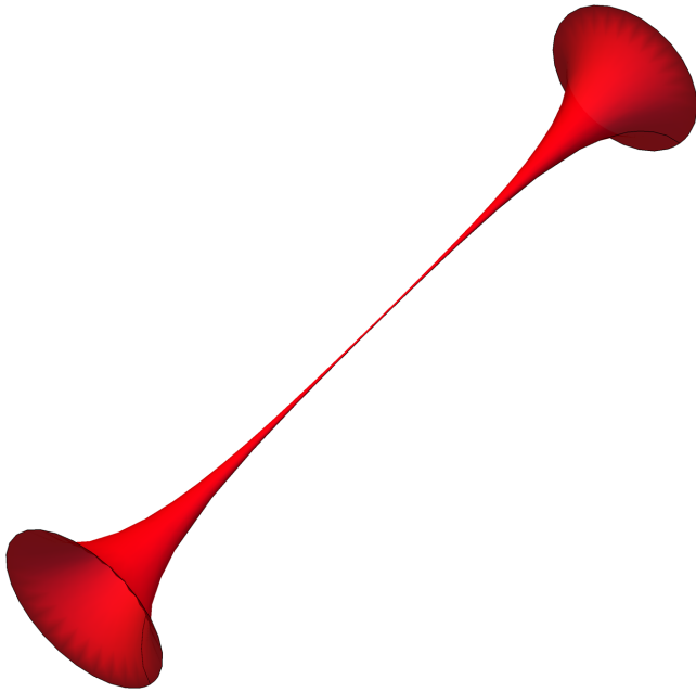
FIG. 4. The hyperbolic pseudosphere for a = 1 , C = 1/100 . Clearly for C/a \rightarrow 0 , the surface tends to two Beltrami pseudospheres joined at the minimum value of \rho , that is \rho_{\min} = C . In the plot, the “Hilbert horizons” are two, and located at the two maximal circles \rho_{\max} = \sqrt{a^2 + C^2} \simeq 1.00005 .
