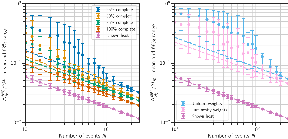
FIG. 8. Fractional uncertainty in H_0 as a function of the number N of the events for the combined H_0 posteriors. The fractional uncertainty in H_0 is defined as the half-width of the 68.3% highest probability density interval divided by 70 \text{ km s}^{-1} \text{ Mpc}^{-1} , and is shown as the plotted dots for all cases. The error bars contain 68% of the scatter arising from different realizations of the events. (left) In purple, red, green, yellow and blue we show the associated host galaxy case (MDA0), complete galaxy catalog (MDA1) case, and the 75%, 50% and 25% completeness cases; we find a fractional H_0 uncertainty of 1.13%, 1.84%, 2.21%, 2.48% and 3.20% respectively for the combined H_0 posterior from 249 events. (right) convergence for MDA3 (event probability proportional to galaxy luminosity), analyzed with luminosity-weighted likelihood (pink) or equally-weighted likelihood (light blue). We find fractional H_0 uncertainties of 4.48% and 5.31% respectively. MDA0 (purple) is included for reference. We plot the expected 1/\sqrt{N} scaling behavior for large values of N for all cases with the dashed lines. This scaling behavior is met by all MDAs as the number of events reaches 249, but for the less informative, lower completeness MDAs the trend is slower to emerge. This is even more evident in MDA3, where the density of galaxies is 100 times greater, producing more potential hosts for each event. This is mitigated somewhat by the effect of luminosity-weighting the potential hosts (pink).
