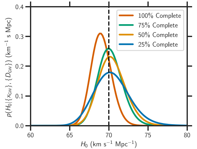
FIG. 5. Comparison of results with varying galaxy catalog completeness. In MDA2, the simulated apparent magnitude threshold is varied to obtain galaxy catalogs of 100%, 75%, 50%, and 25% completeness. The corresponding posterior probability densities on H_0 using all 249 events are shown in red, green, yellow, and blue respectively.
