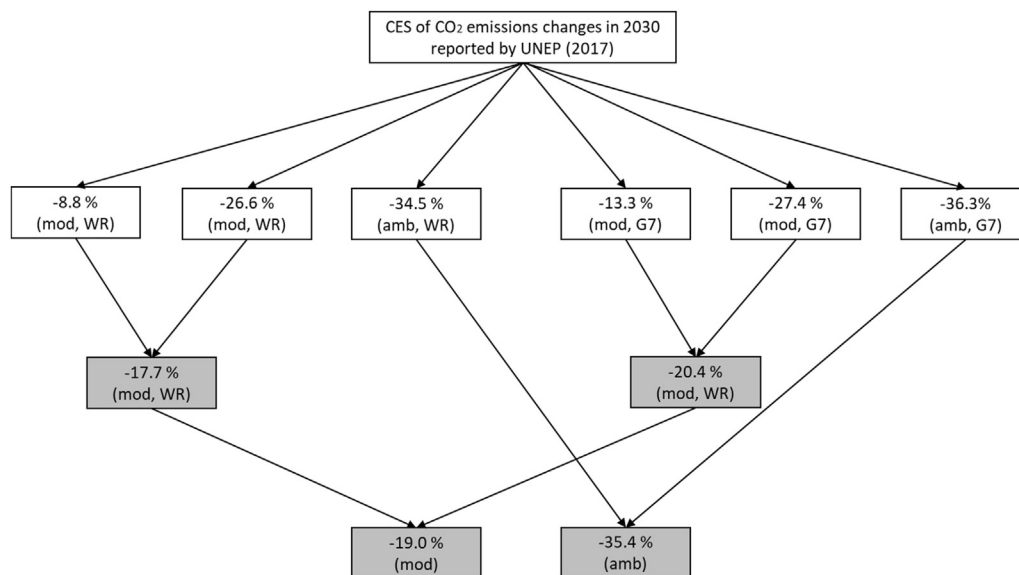
Fig. 2. Example of data harmonization using the values reported by UNEP (UNEP, 2017). Numerical values represent changes in CO 2 . Texts in parenthesis indicate scenario type and country/region. Abbreviations: mod = moderate scenarios; amb = ambitious scenarios; WR = world; G7 = Group of Seven (i.e. Canada, France, Germany, Italy, Japan, the United Kingdom and the United States). Solid blocks in grey indicate the calculated average of each scenario type. Note that not all studies cover all years from 2020 to 2050 and not all studies cover the three types of impact (GDP, employment, and CO 2 ). File results_time_ser.xlsx in Supplementary Material presents the details of how many ambitious and moderate CESs are available for each year and impact type.
