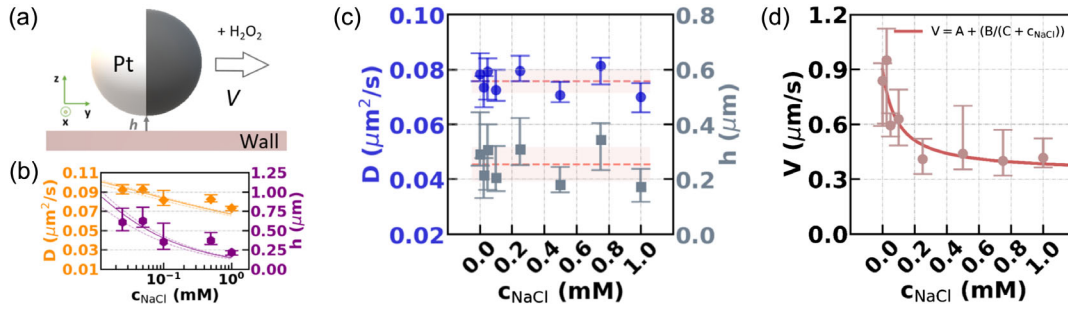
FIG. 1. Salt-dependent motion above a planar wall. (a) Schematic of the experiment. We obtain the swimmer-wall separation h from the measured translational diffusion coefficient D of the swimmer and its theoretically predicted dependence on wall separation. (b)–(d) Effect of salt concentration c_{\text{NaCl}} on the motion of 2.77 \pm 0.08 \mu\text{m} colloids with 4.4 \pm 0.2 \text{ nm} Pt. All reported values are medians, and error bars denote first quartiles. (b) Diffusion coefficient (orange diamonds) and separation (purple hexagons) in the Brownian state in water with c_{\text{NaCl}} . Lines show theoretical predictions based on balancing electrostatics and gravity. (c) Diffusion coefficient (circles) and separation (squares) in the active state in aqueous 10% \text{H}_2\text{O}_2 with c_{\text{NaCl}} . Dotted lines indicate mean values. (d) Speed decrease in 10% \text{H}_2\text{O}_2 with c_{\text{NaCl}} . The solid line is a least-squares fit with V = A + [B/(C + c_{\text{NaCl}})] , where A is 0.35 \pm 0.09 \mu\text{m/s} , the remaining speed in high salt, B is a prefactor, and C is 0.09 \pm 0.07 \text{ mM} , the ion concentration already present in solution, following from ionic diffusio-osmosis along the wall.
