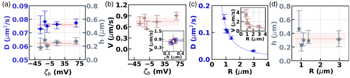
FIG. 2. Swimmer base zeta potential and size dependence of propulsion above a planar wall. All reported values are medians, error bars denote first quartiles, and dotted lines represent mean values. All experiments were performed in aqueous 10% \text{H}_2\text{O}_2 . (a),(b) The base zeta potential \zeta_b of TPM colloids with diameters between 2.70 \pm 0.06 and 2.77 \pm 0.08 \mu\text{m} and Pt coating thicknesses \approx 4.4 \pm 0.2 \text{ nm} was varied through surface functionalization. (a) Diffusion coefficient (circles) and separation (squares) with \zeta_b . (b) Speed for the same \zeta_b range as in (a). The inset shows speed with separation (purple circles), with the white circle marking the intersection of mean values and the rectangle around it denoting standard deviations. (c),(d) Variation of the radius R of active TPM spheres with similar \zeta_b and Pt (coating thickness \approx 4.5 \pm 0.2 \text{ nm} ) affects (c) the diffusion coefficient and (d) swimmer-wall separation. The inset in (c) shows swim speed with R . Solid lines in (c) are fits with a/R^b with a = 0.120 \pm 0.004 \mu\text{m}^3/\text{s} and b = 1.3 \pm 0.2 (main) and the expected a/R [29] with a = 2.2 \pm 0.4 \mu\text{m}^2/\text{s} (inset). The dotted line in (d) shows mean separation ( 0.32 \pm 0.08 \mu\text{m} ).
