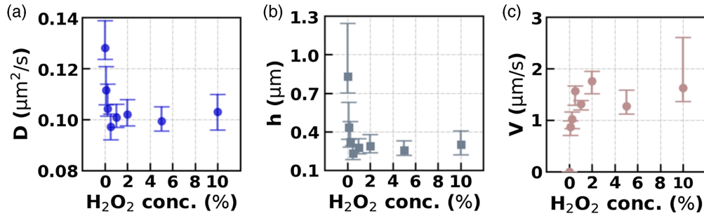
FIG. 3. Activity-induced ypsotaxis. (a) Diffusion coefficient D with increasing \text{H}_2\text{O}_2 (fuel) concentration. (b) Equivalent swimmer-wall separation h for the same fuel concentration range. (c) Swim speed V for the same fuel concentration range as in (a),(b). All experiments were performed using 2.23 \pm 0.11 \mu\text{m} diameter TPM spheres with 4.5 \pm 0.2 \text{ nm Pt} . All reported values are medians and error bars denote first quartiles.
