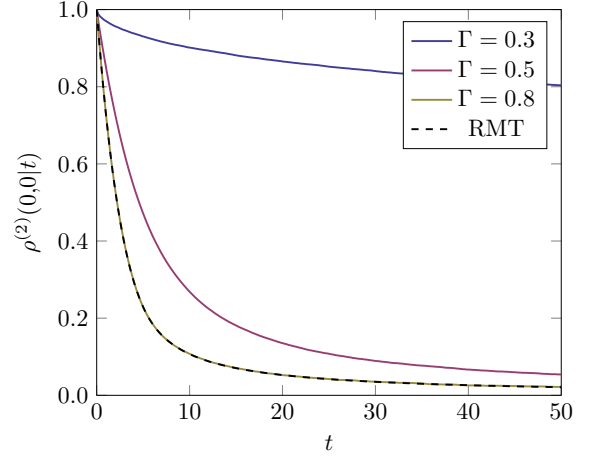
FIG. 1. Numerically obtained \rho^{(2)}(0, 0|t) as a function of t at system size L = 12 for \Gamma = 0.3 (top curve), \Gamma = 0.5 (middle curve), and \Gamma = 0.8 (lower curve). The dashed line displays the random matrix (RMT) theory prediction for fully ergodic systems.
