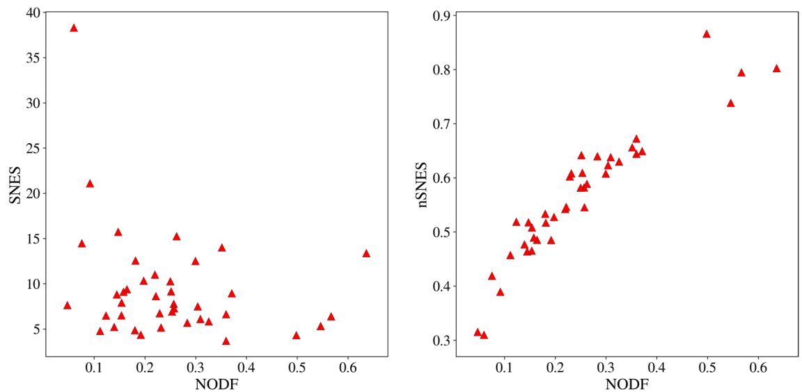
Figure 1. NODF versus SNES (left) and versus nSNES (right) for the 40 networks of the Bascompte dataset. Spearman correlation coefficients are, respectively, -0.23 and 0.96 . In fact similar relations hold when considering sNODF instead of NODF: evidences can be found in the Supplementary Fig. A.
