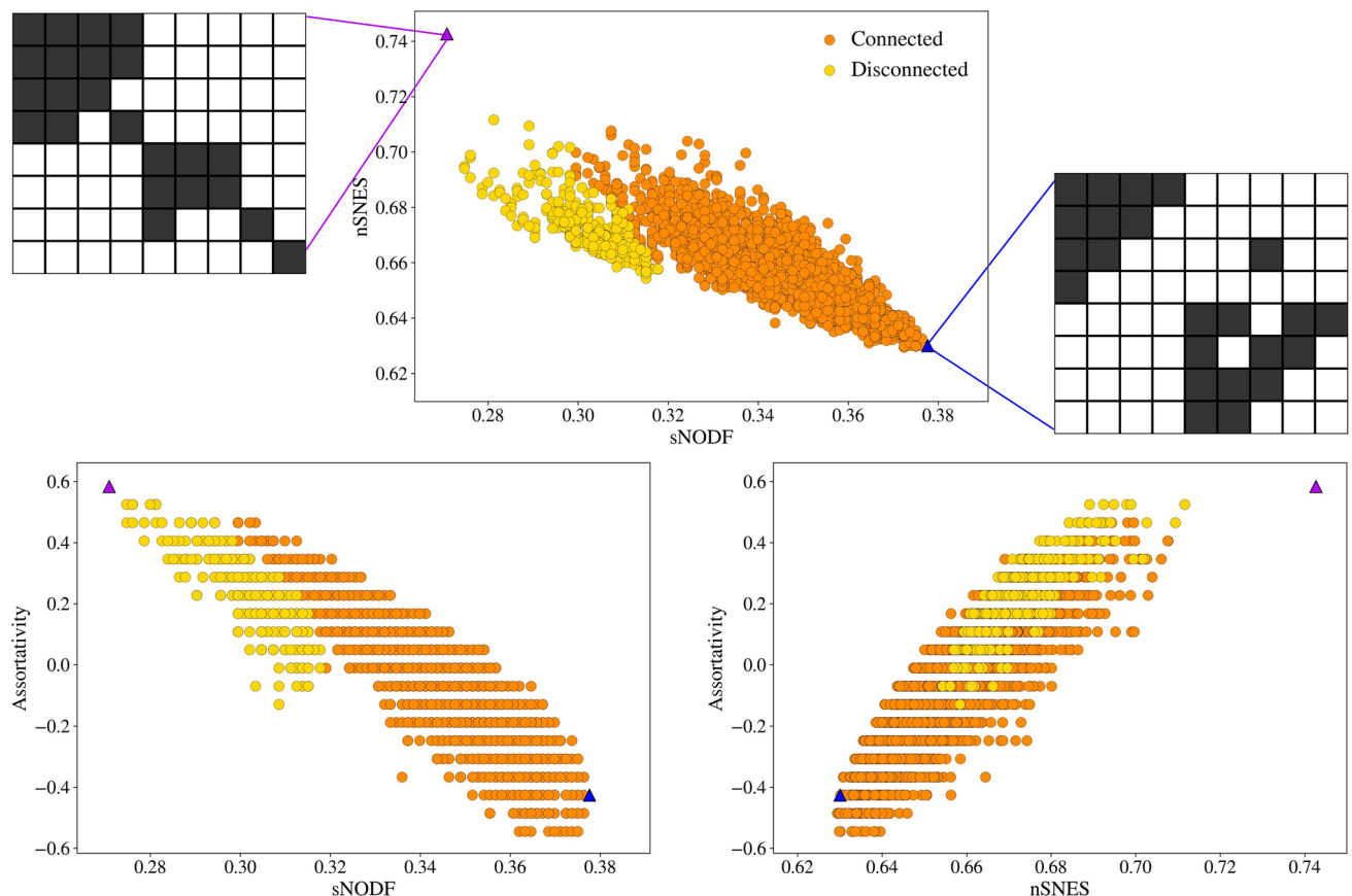
Figure 6. Top: a sample from the microcanonical configuration model ensemble with the relative scores of nSNES and sNODEF. Bottom: the same sample with scores of sNODEF against assortativity (left), nSNES against assortativity (right). Different colours are used for sampled networks that result connected or disconnected. The highlighted networks have high values of nSNES or sNODEF, and show that for their extreme values, the systems can be disconnected (left) or barely connected (right). The left matrix, with a high nSNES, has a really assortative configuration, while the right one has a high sNODEF and is highly disassortative. We do not exclude disconnected networks in our analysis since it could be a possible configuration for an ecological system.
