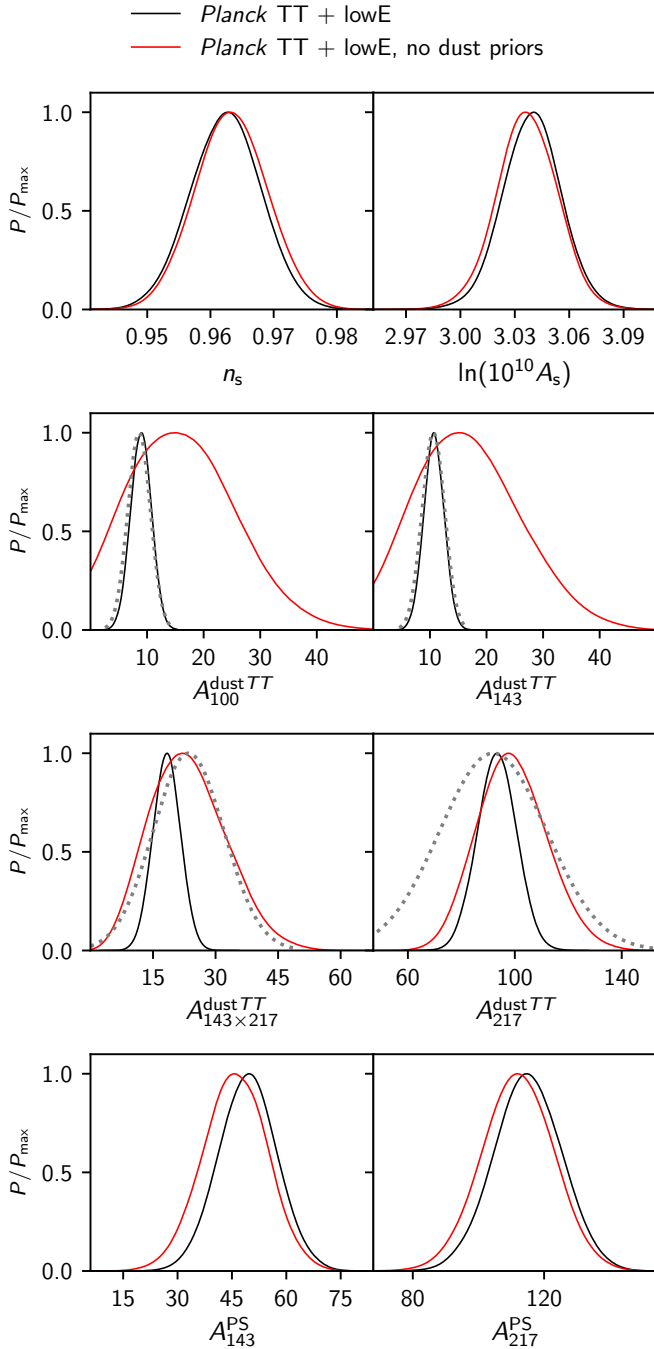
Fig. 40. One-dimensional posterior distributions for cosmological and nuisance parameters using TT +SimA11. The black line shows the baseline set of results, which adopts priors on the dust amplitudes. The red lines show the case when we leave the amplitudes free to vary; these are in good agreement with the priors set in the baseline, which are indicated with grey dotted lines. As a consequence, leaving the dust amplitudes free to vary without priors has small to negligible impact on other parameters.
