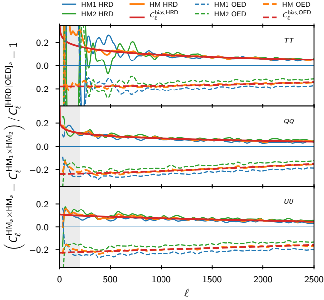
Fig. 48. Correction ( C_{\ell}^{\text{bias}} ) for the noise estimates based on HRDs (solid lines) and OEDs (dashed lines), as described in Eqs. (35) and (36). Blue and green lines show the two contributions to the bias estimates (i.e., for HM1 and HM2), showing that the bias is similar enough in each so that we can use the mean for the correction (orange line). The model fit (red) is obtained by restraining the fit to the non-shaded region ( \ell > 200 ). As we found in PPL15, HRD noise estimates are found to be biased low (due to correlations between half-ring maps, as explained in Planck Collaboration VI 2014). OED noise estimates, on the other hand, are biased high (in particular in polarization). Once the corresponding correction is applied to either case (HRD or OED), the overall noise models are similar. We only present here the 100 GHz channel results where the effect is the most striking. OEDs have very low anti-correlation for TT at 143 GHz and a slight correlation at 217 GHz, while the QQ and UU equivalents are still anticorrelated at all frequencies.
