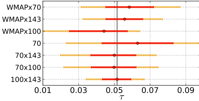
Fig. 18. Whisker plot showing best-fit values and 68% and 95% confidence levels for \tau when combining various Planck and WMAP channels. The vertical line shows the best-fit value from 100 \times 143 .
