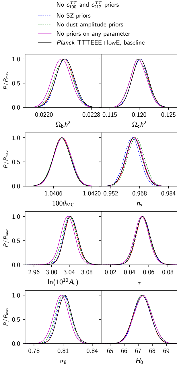
Fig. 76. Impact of lifting priors on \Lambda CDM cosmological parameters. We show results obtained when lifting the TT inter-frequency parameters c_{100}^{TT} and c_{217}^{TT} described in Sect. 3.3.4 (dashed red), when lifting the SZ amplitude priors described in Sect. 3.3.1 (dashed blue), and when lifting the dust amplitude priors in TT and TE , while allowing the dust-amplitude values in EE to vary freely (dashed green). We also show the impact of letting all of the nuisance parameters vary freely (keeping only a prior on the overall calibration y_p , as given in Eq. (39), solid magenta). The baseline TTTEEE+SimAll case is in solid black. In all these cases, shifts with respect to the baseline are smaller than 0.5\sigma .
