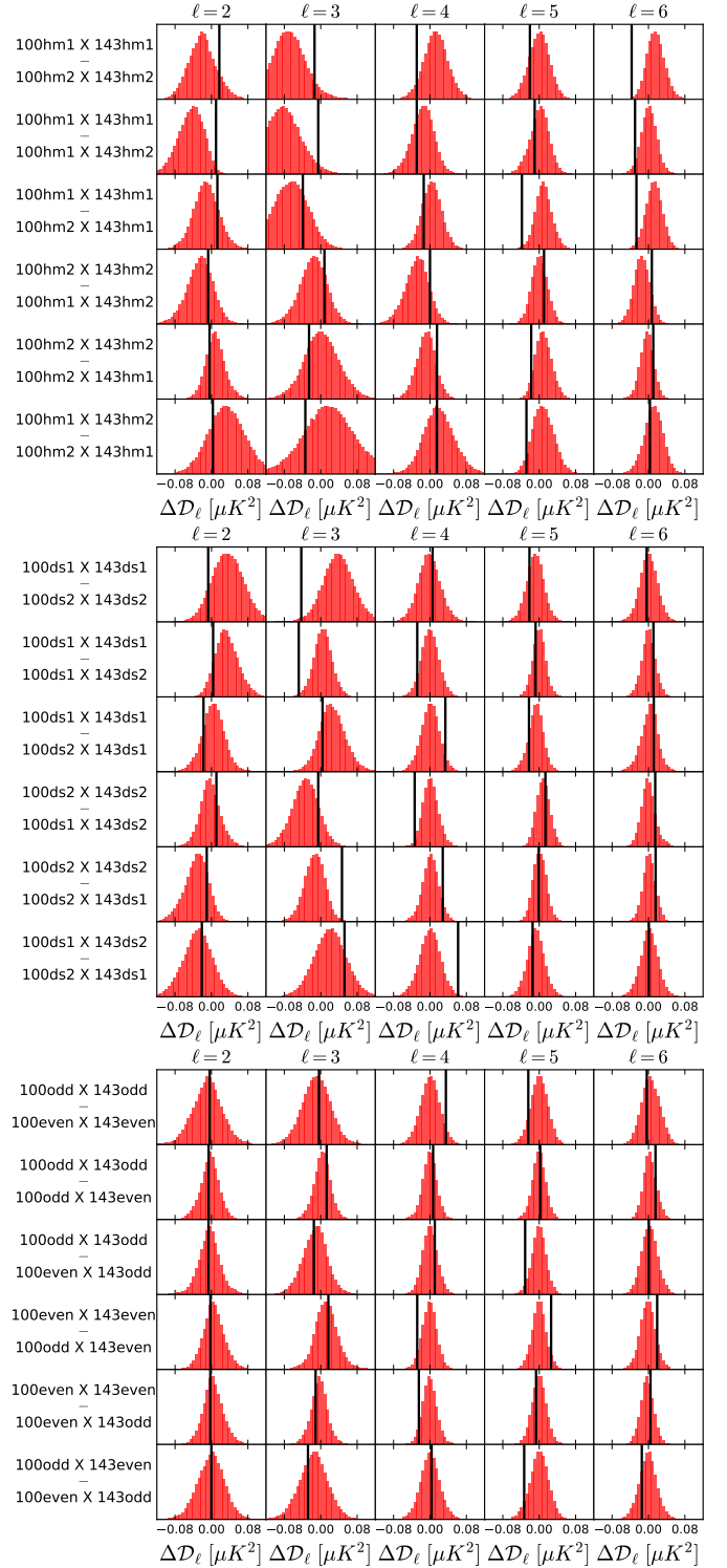
Fig. 10. Difference, \Delta\mathcal{D}_t , between spectra for different data splits (vertical line), compared with the distribution of the difference in FFP10 simulations (histograms).
