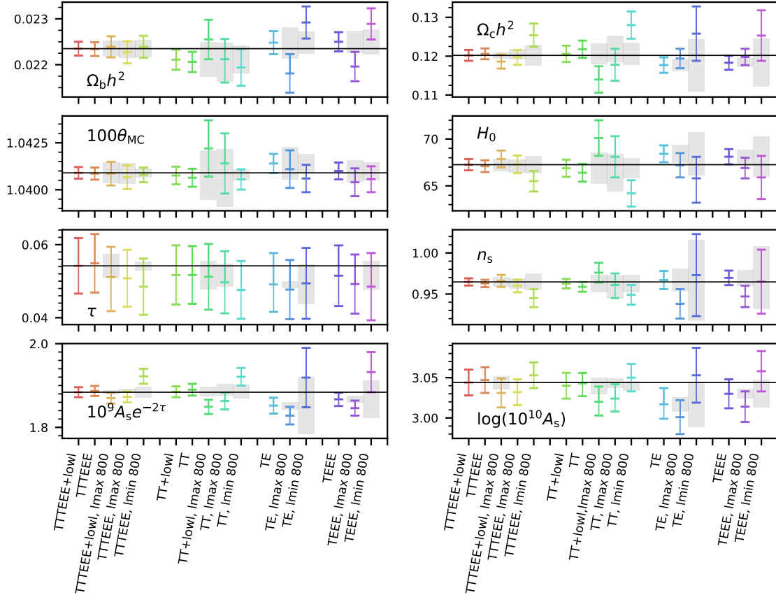
Fig. 81. Marginal means and 68% error bars on the cosmological parameters for Plik TT , TE , TEEE , and TTTEE , combined with SimAll and in some cases low lTT (as indicated in the labels), in the full multipole range and for two different multipole cuts, namely \ell < 800 and \ell > 800 .
