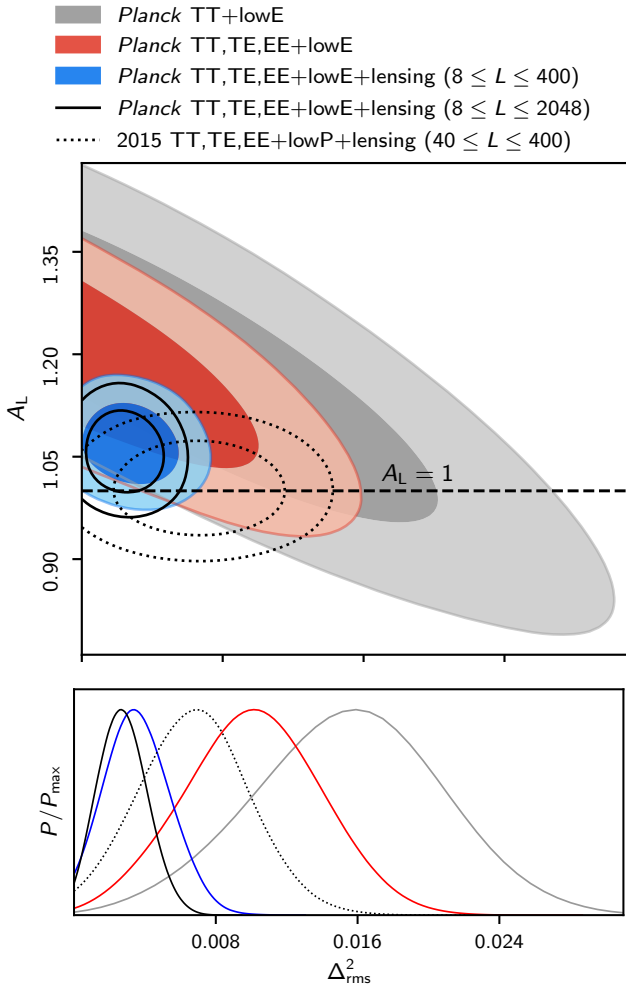
Fig. 47. Degeneracy between A_L and \Delta^2_{\text{rms}} in the \Lambda\text{CDM}+A_L+\text{CIP} model (top panel) and constraints on \Delta^2_{\text{rms}} in the \Lambda\text{CDM}+\text{CIP} model, where A_L = 1 (bottom panel).
