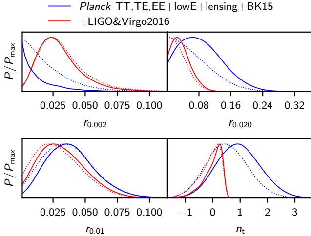
Fig. 4. Posterior probability density of the tensor-to-scalar ratio at two different scales in the \Lambda CDM+ r_{0.002} + r_{0.02} model, i.e., when the inflationary consistency relation is relaxed ( top panels ). The solid contours show the results when r_{0.002} and r_{0.02} are used as sampling parameters with uniform priors, which leads to non-uniform priors for the derived parameters r_{0.01} and n_t ( bottom panels ). The dotted contours indicate the results after weighting the posterior by the Jacobian J = r_{0.01}/[r_{0.002}r_{0.02} \ln(0.02/0.002)] of the transformation (r_{0.002}, r_{0.02}) \rightarrow (r_{0.01}, n_t) , giving the result we would have obtained had we assigned uniform priors on r_{0.01} and n_t .
