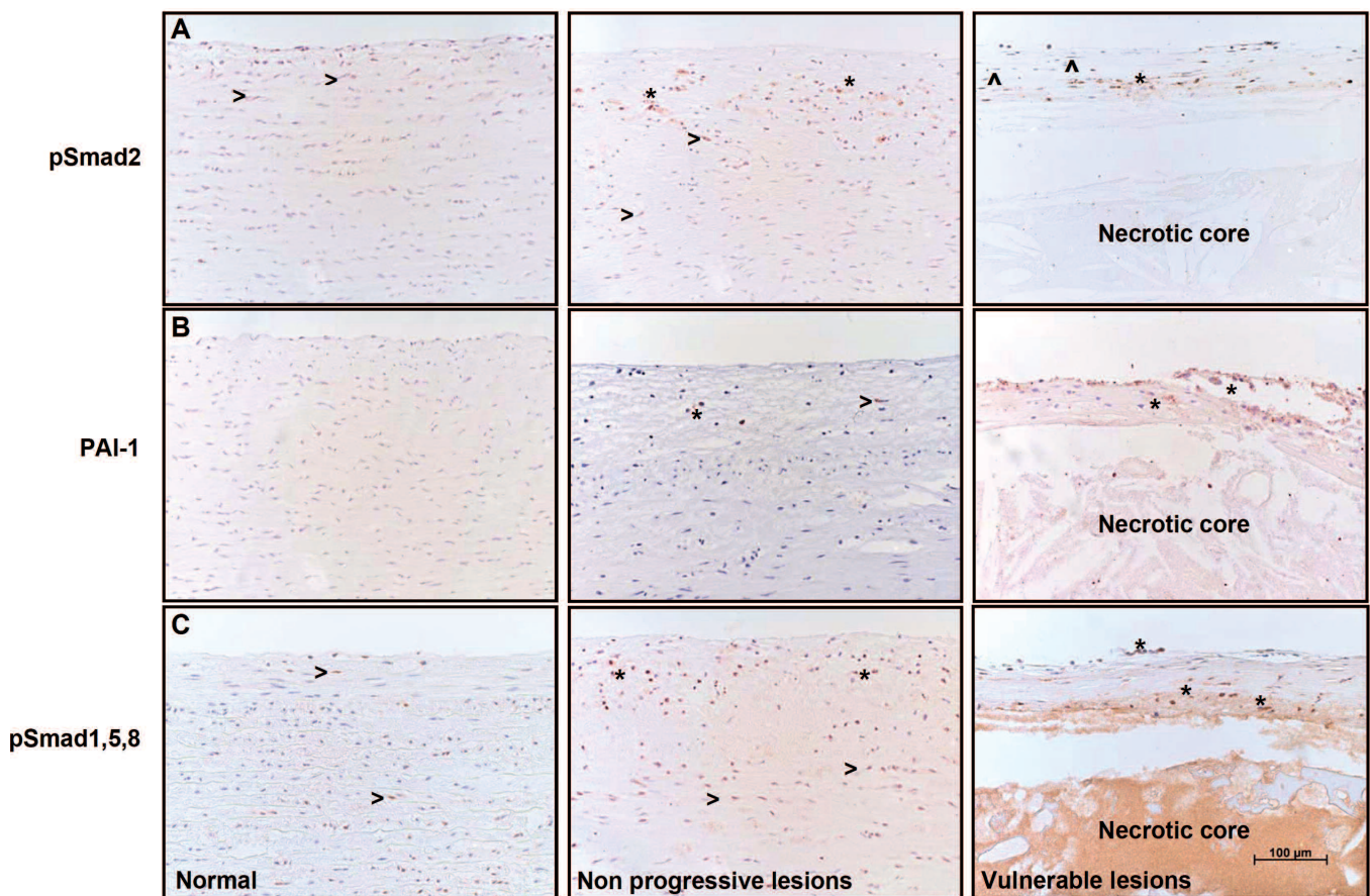
Fig. 2. Expression of pSmad2, PAI-1 and pSmad1,5,8 in the human aorta. A. Within the normal aortic wall only few SMCs stain positively for pSmad2. Macrophages and SMCs expressing pSmad2 are abundantly present within the intima and media of non-progressive lesions. The SMCs resident in the thinning cap of the vulnerable lesions remain devoid of Smad2 activation. B. Minimal PAI-1 expression was found in the intimal layer of normal aortic tissue. In the vulnerable lesions the thin fibrous cap lacks PAI-1 positive SMCs, whereas almost all macrophages stained positive for PAI-1. C. Early non-progressive lesions are characterized by a significant increase in Smad1,5,8 positivity. The vulnerable thin cap mainly consists of pSmad1,5,8 expressing monocytes and/or macrophages. All images were taken at 20x magnification and correspond with the indicated 100 \mu m scalebar. (>: Intimal or medial positively stained SMCs; *: Positively stained monocytes or macrophages; ^: Intimal SMCs devoid of Smad2 activation).
