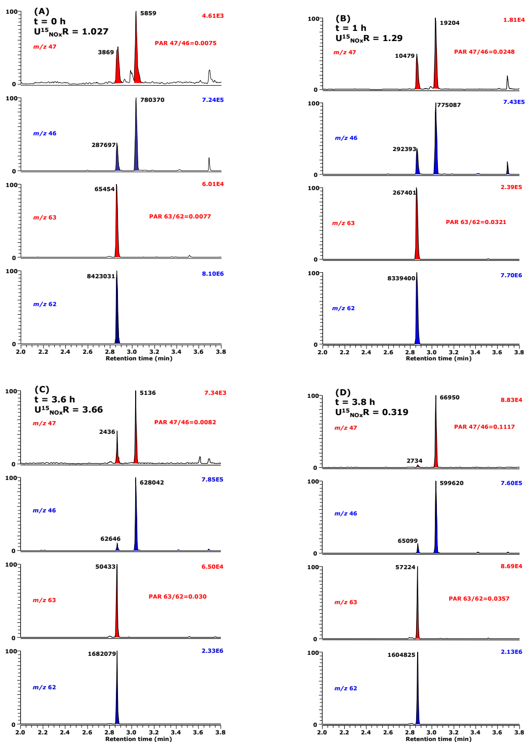
Fig. S3. GC-MS chromatograms from analyses of spot urine samples collected before and after [ ^{15}\text{N} ]nitrite sodium and acetazolamide intake by a healthy female subject (age, 25 years) (Tsikas et al. 2010b). The volunteer drank two times [ ^{15}\text{N} ]nitrite sodium dissolved in drinking water (0.31 \mu\text{mol/kg} each) and took once acetazolamide (5.4 mg/kg bodyweight). The first [ ^{15}\text{N} ]nitrite intake was ingested at the time point “zero” (0 h, panel A). U^{15}_{NOx}R is calculated by dividing the peak area ratio (PAR) of m/z 63
