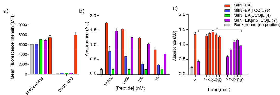
Figure 2. Optimization of in vitro deprotection of the trans -cyclooctene protected epitope SIINFEKL. (a) Binding affinity (MFI) of the caged epitopes, compared to SIINFEKL, to cell surface H2–K b at low temperatures of the TAP deficient cell-line RMA-S. Analysis was performed with anti H2–K b and H2–K b –SIINFEKL specific antibody (25-D1-APC). SIINFEK[mbTCO]L (7 purple), CCO (4, green), and TCO (5, blue), SIINFEKL (red). (b,c) Deprotection of caged peptides (4, 5, 7) using DC2.4 cells as APCs and B3Z cells as T-cells. T-cell activation was compared to wild-type response (SIINFEKL; red) by measuring absorption (AU) of beta-galactosidase-directed CPRG hydrolysis. All experiments have been done twice in triplicate; error bars represent the standard error of the mean. (b) Deprotection of CCO (4, green), TCO (5, blue), and mbTCO (7, purple) in the presence of 50 \mu M 3,6-dimethyltetrazine (8) for 30 min and indicated peptide concentrations. (c) Deprotection of 100 nM mbTCO (7) after incubation with 50 \mu M 8 for the indicated times. After 1 min incubation, a significant ( p = 0.04 ) T-cell response could already be detected.
