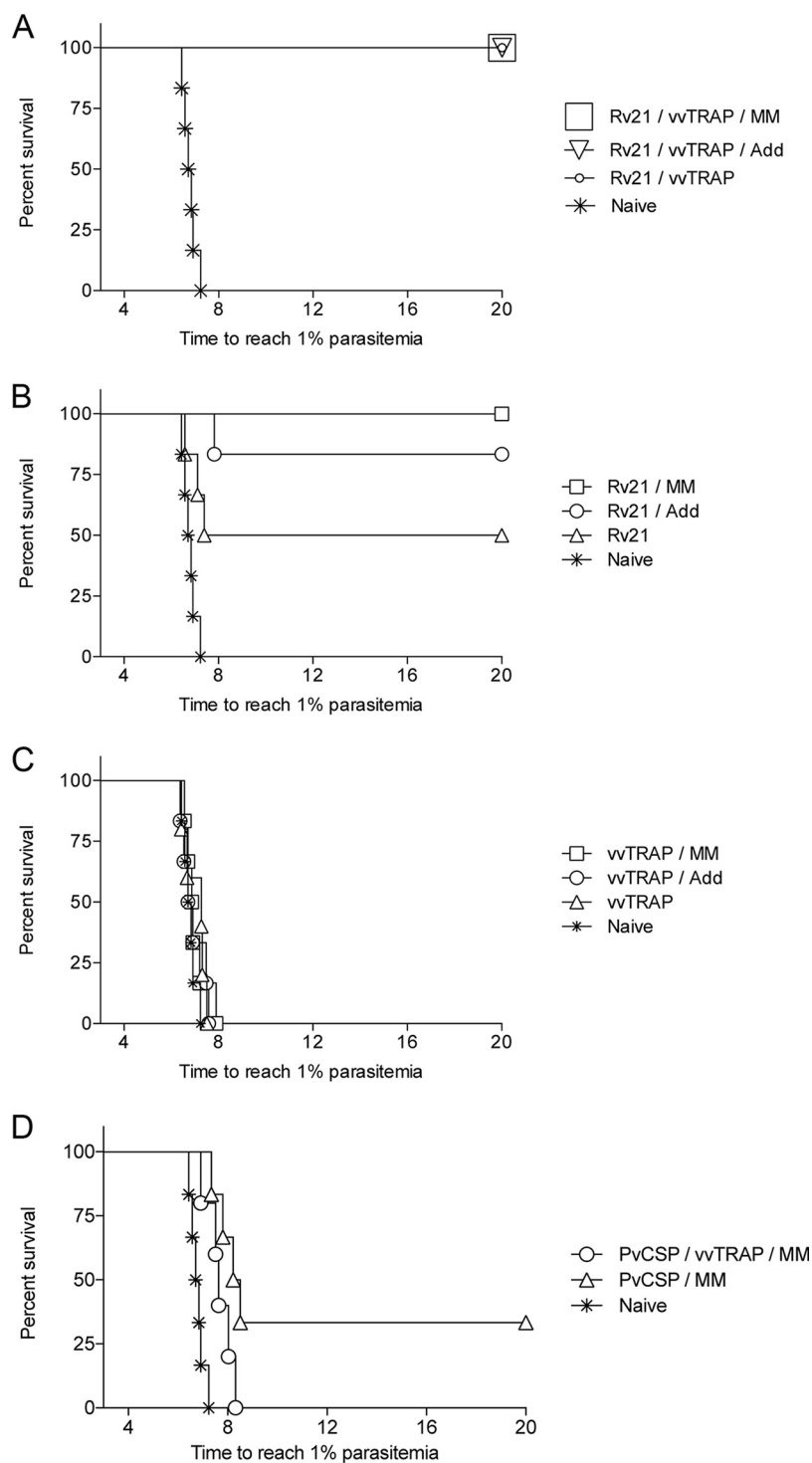
FIG 4 Protective efficacy against a transgenic sporozoite challenge using a combination of the Rv21 and vvTRAP, in the presence of Matrix-M or AddaVax adjuvants. Inbred BALB/c mice ( n = 6 per group) vaccinated with Rv21 and/or vvTRAP as described in Table 1 were challenged by intravenous administration of transgenic P. berghei PvCSP-VK210/PvTRAP double-replacement parasites using a stringent challenge with 2,000 sporozoites. (A) Efficacy of a vaccine consisting of Rv21 combined with either vvTRAP or of vvTRAP plus the adjuvant Matrix-M (MM) or AddaVax (Add). (B) Efficacy of Rv21 in the presence of chemical adjuvants. (C) Efficacy of a prime-boost vaccination regimen using vvTRAP. (D) Efficacy of a P. vivax CSP protein in combination with vvTRAP and Matrix-M adjuvants.
