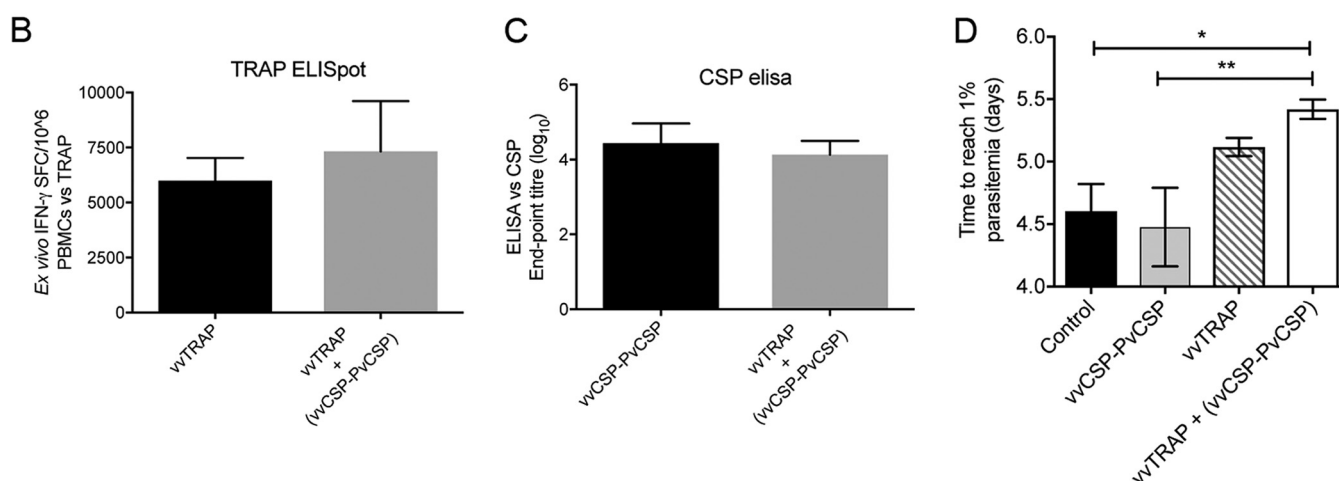
FIG 2 Immunogenicity and protective efficacy of a combination P. vivax CSP-VK210 with adenoviral or MVA viral vectors expressing P. vivax TRAP (vvTRAP). (A) Inbred female BALB/c mice ( n = 7 to 8/group) were primed with PvCSP-VK210 viral vector (vv) followed by the PvCSP protein (vvCSP-PvCSP), ChAd63-MVA viral vector expressing PvTRAP (vvTRAP), or their combination (vvTRAP+vvCSP-PvCSP). (B) Two weeks postboost ex vivo IFN- \gamma ELISpot responses were measured upon restimulation of whole-blood PBMCs with three subpools of peptides representing the full-length PvTRAP. Values are means and standard errors of the means. (C) An endpoint titer ELISA was done to quantify anti-PvCSP-VK210 antibodies. Bars indicate median responses. (D) Two weeks after the last vaccination, animals were challenged by intravenous injection of 2,000 double-transgenic P. berghei PvCSP-VK210 and PvTRAP sporozoites. Blood stage infection was recorded over three consecutive days starting at day 5 postchallenge, and a linear regression model predicting time to 1% blood stage parasitemia for individual animals was applied, showing a significant delay in the vvTRAP+vvCSP-PvCSP group that received a combination vaccine compared to time for the other treatment groups. Values are means and standard errors of the means. * P < 0.05 ; ** P < 0.01 (Mann-Whitney test comparing two groups).
