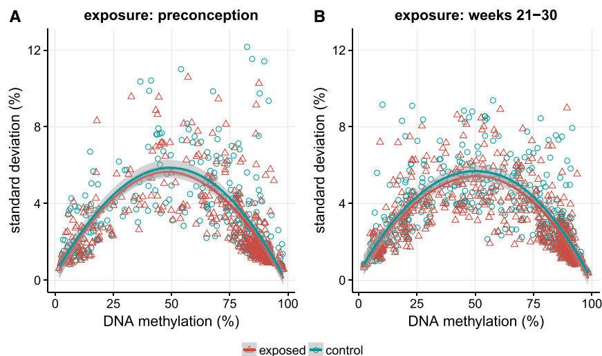
Figure 3. Empirical Data for the Relationship between Mean and SD of DNAm Data in the Dutch Hunger Winter Families Study
