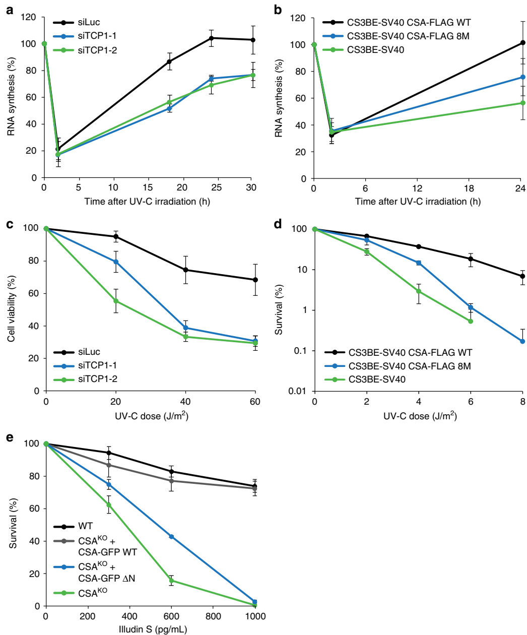
Fig. 6 Loss of TRiC reduces RRS and protection against UV damage. a TCP1 loss reduces RNA synthesis recovery following UV-C irradiation. VHI0-hTert cells were transfected with the indicated siRNAs and UV-C irradiated (10 J/m 2 ). RNA synthesis was measured by means of EU incorporation at the indicated time points after UV. RNA synthesis levels were normalized to those in non-irradiated cells, which were set to 100%. Data represent the mean ± SEM of four independent experiments. b Expression of CSA-FLAG 8M shows reduced RNA synthesis recovery as compared to expression of CSA-FLAG WT. As in a , except that CS3BE-SV40 cells expressing CSA-FLAG WT or CSA-FLAG 8M were used. Data represent the mean ± SEM of four independent experiments. c TCP1 loss renders cells hypersensitive to UV damage. VHI0-hTert cells were transfected with the indicated siRNAs, UV-C irradiated at the indicated doses and 72 h later assayed for viability using alamarBlue®. Data represent mean ± SEM of four independent experiments. d Expression of CSA-FLAG 8M in CS3BE-SV40 cells fails to rescue UV-sensitivity. CS3BE-SV40 cells stably expressing CSA-FLAG WT or CSA-FLAG 8M were UV-C irradiated and clonogenic survival was measured. Data represent mean ± SEM of three independent experiments. e CSA WT, but not CSA ΔN, complements the Illudin S sensitivity of CSA knockout (KO) U2OS cells. The indicated cells were treated with different concentrations of Illudin S and clonogenic survival was determined. Data represent mean ± SEM of three independent experiments
