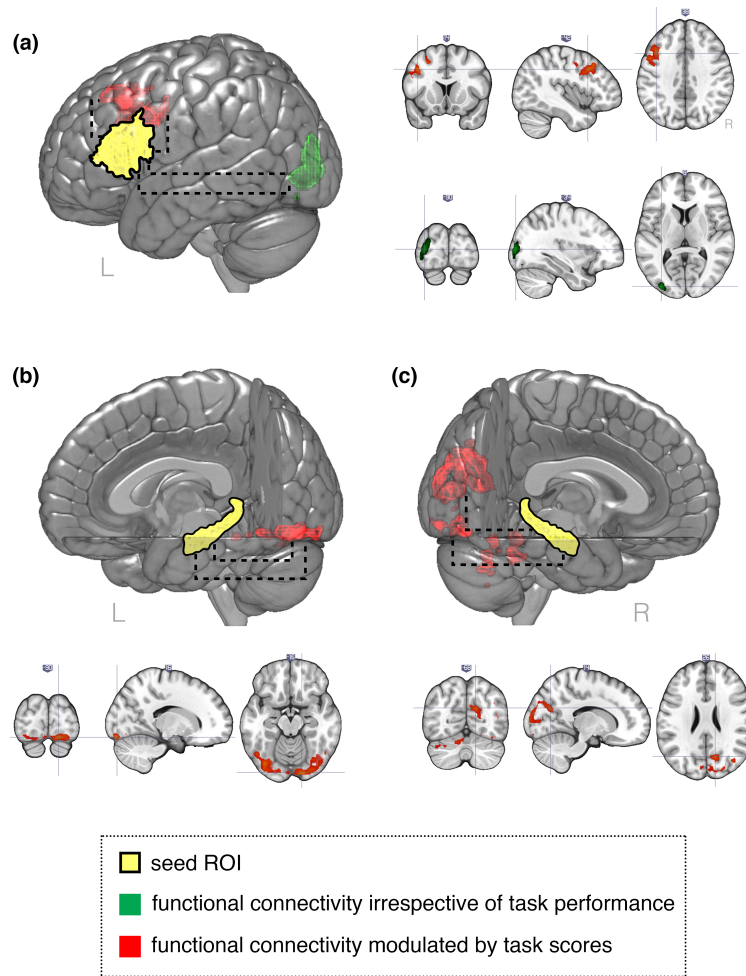
Figure 3 Results of the PPI analysis investigating time-invariant functional connectivity of the four seed ROIs. Represented are the mean connectivity maps (Z (Gaussianised T/F) statistic images) of each seed ROI: a) Left BA 44/45 (Broca's region), (b) Left Hippocampus, (c) Right Hippocampus; the seed ROI localised in the right BA 44/45 did not yield any significant clusters. Results are displayed at p < .05 , Bonferroni-corrected. In yellow, the seed ROIs are marked; in green results of the contrast testing for mean functional connectivity of the whole group irrespective of task performance; in red, the connectivity modulated by the task performance is shown. Brain activations are displayed using MRICroGL ( http://www.mccauslandcenter.sc.edu/mricrogl/ ).
