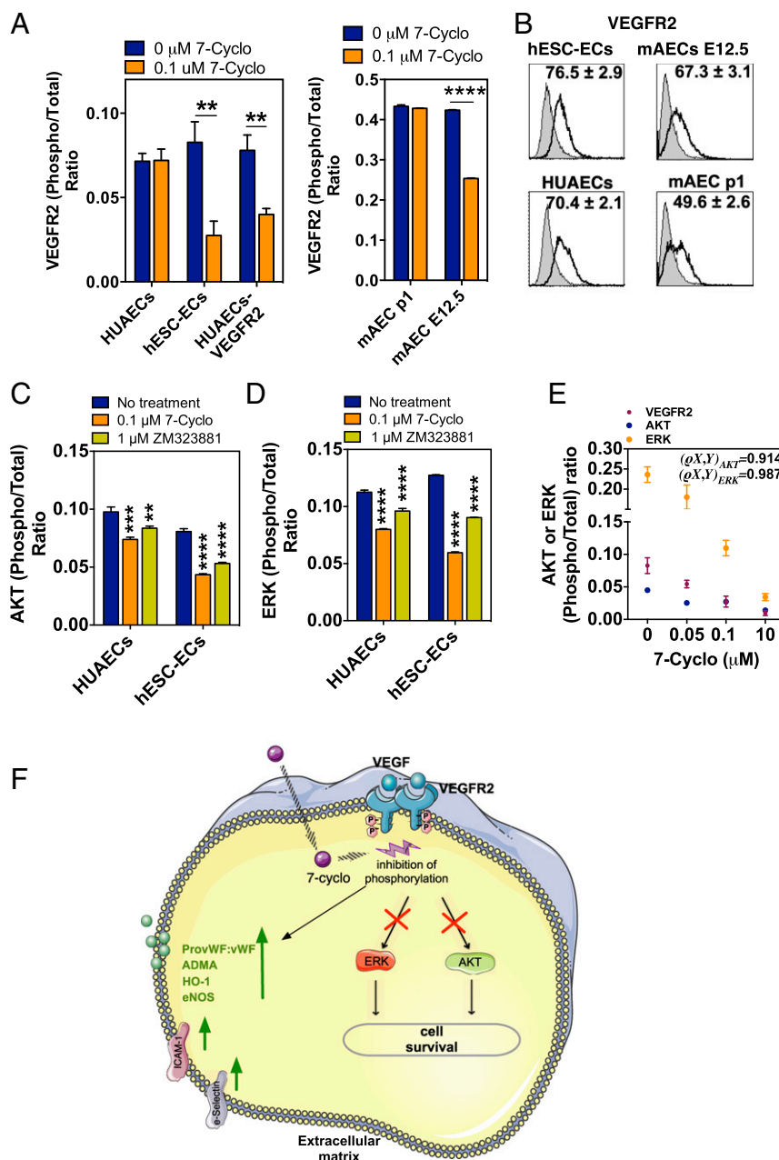
Fig. 6. Effect of 7-Cyclo in VEGFR2. (A) Phosphorylation of VEGFR2 in human and mouse embryonic and postnatal cells treated with 0 or 0.1 μM 7-Cyclo for 72 h (by ELISA). Results were normalized by the total form of protein and indicate mean ± SEM ( n = 4 ). HUAECs-VEGFR2 cells are HUAECs overexpressing VEGFR2. Statistical analyses between groups were performed by an unpaired t test. (B) VEGFR2 is more highly expressed in embryonic cells (hESC-ECs or mAECs E12.5) than in postnatal cells (HUAECs or mAECs p1), either in human or mouse cells. Percent of positive cells was calculated based on the isotype controls (gray plot) and is shown in the histogram plots. Values in histogram plots indicate mean ± SEM ( n = 3 ). (C and D) Effect of 7-Cyclo (0.1 M) and ZM323881 (1 M; VEGFR2-specific inhibitor) in the phosphorylation of AKT (C) and ERK (D) in hESC-derived ECs and HUAECs for 15 min (by ELISA). Results were normalized by the total form of protein and indicate mean ± SEM ( n = 4 ). Statistical analyses between experimental group “no-treatment” and the other two groups was performed by one-way ANOVA test followed by a Newman-Keuls multiple comparisons test. (E) Correlation between the inhibition of VEGFR2 phosphorylation and the inhibition of AKT ( P = 0.914 ) or ERK ( P = 0.987 ) phosphorylation. Correlations indicate a strong relationship between both events. Values indicate mean ± SEM ( n = 4 ). (F) Schematic representation of the impact of 7-Cyclo in embryonic ECs. The 7-Cyclo inhibits VEGFR2 phosphorylation, leading to the inhibition of downstream pathways involved in cell proliferation and survival (ERK and AKT pathways). The 7-Cyclo also increases the expression of the molecules involved in vascular injury such as ADMA, propeptide vWF, eNOS, ICAM-1, eSelectin, and HO-1. * P < 0.05 ; ** P < 0.01 ; *** P < 0.001 ; **** P < 0.0001 .
