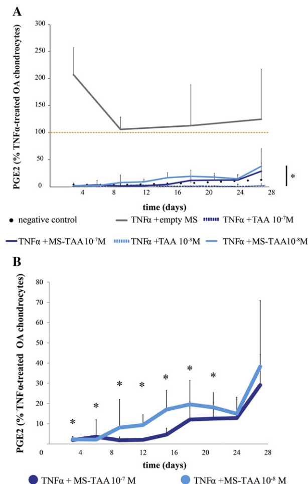
Fig. 2. PGE 2 production was inhibited during the total culture period upon TAA treatment, regardless of dose and formation, compared to chondrocytes treated solely with TNFα (100%, orange dotted line) except in the presence of empty microspheres (grey solid line). Negative control indicates chondrocytes without TNFα (black dotted line), TNFα + TAA 10 -7 M (dark blue dotted line) and TNFα + TAA 10 -8 M (light blue dotted line) represent free 0.1 or 0.01 μM TAA, respectively, added to the culture medium. Corresponding TAA dosages in microspheres are indicated with TNFα + MS-TAA 10 -7 M (dark blue solid line) and TNFα + MS-TAA 10 -8 M (light blue solid line). Results are shown as average mean ± SD for three donors with six replicates per donor. *p < 0.05.
