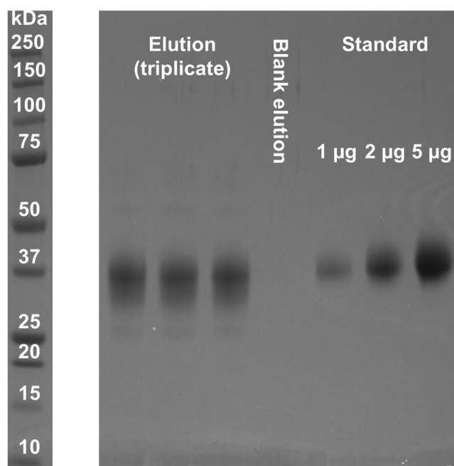
Figure 3. EPO purity after affinity purification. From left to right: Eluate of the affinity purification from CCS (triplicate); Eluate without prior application of CCS (negative control); EPO standard in ascending order of amounts (1, 2 and 5 µg). The three different bands of each affinity purification of CCS were excised and subjected to a standard protein identification workflow (see Supporting Information Table S3).
