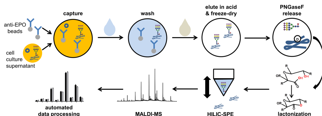
Figure 1. The CCS was mixed and incubated with anti-EPO beads in a 96-well filter plate. After washing, pure proteins were eluted in HCl and freeze dried. Glycans were prepared by PNGaseF release without additional denaturation, lactonization for stabilization and HILIC-SPE. MALDI-TOF-MS analysis in reflectron positive mode yielded high quality spectra which were automatically quantified with MassyTools.
