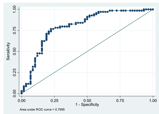
Fig. 3 Post-estimation of ROC-curve after logistic regression analysis, CCP2, and CCP3
