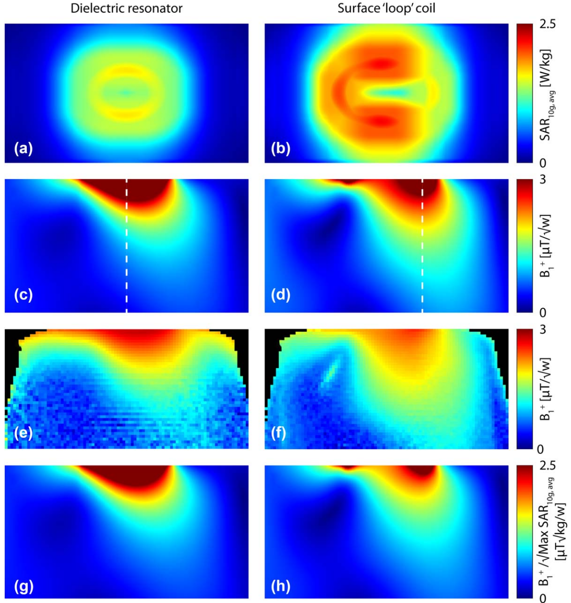
FIG. 4. (a–b) Maximum intensity plot of the simulated SAR_{10g, avg} of the DRA and surface coil normalized to 1W input power placed on a 120 \times 120 \times 210 \text{ mm}^3 phantom ( \epsilon_r = 80 , \sigma = 0.40 \text{ S/m} ). (c–d) Simulated B_1^+ distribution normalized to 1W input power in the same phantom. (e–f) B_1^+ distribution measured using the dual refocusing echo acquisition mode sequence normalized to 1W input power. (g–h) Simulated B_1^+ distribution normalized to the maximum SAR_{10g, avg} , 1.62 W/kg, and 2.20 W/kg for the DRA and surface coil, respectively. DRA, dielectric resonator antenna; SAR, specific absorption rate.
