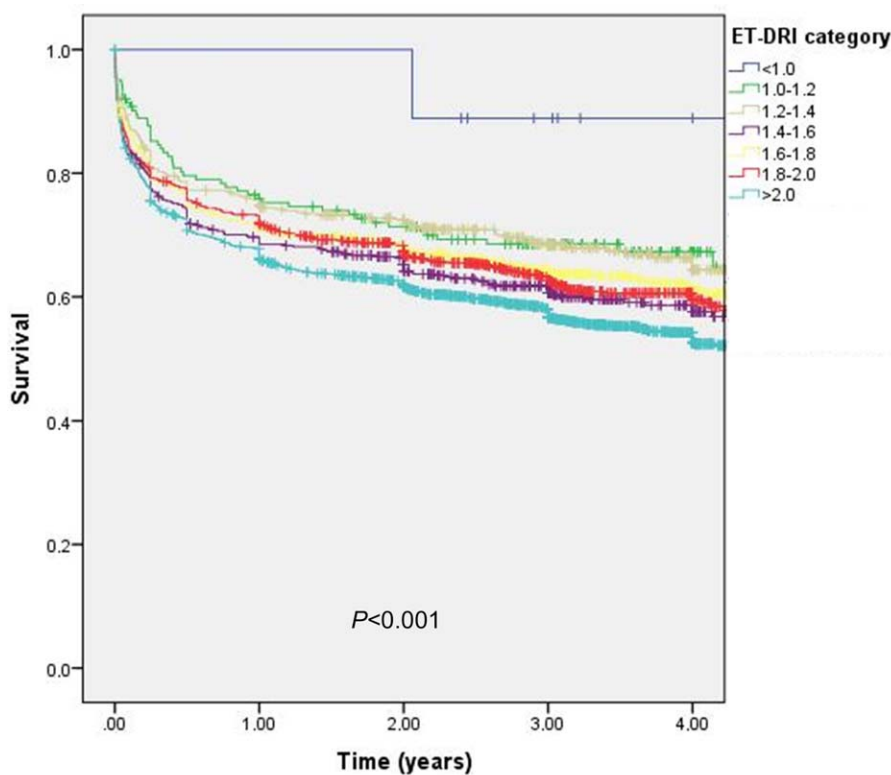
Figure 2. Kaplan-Meier survival analysis of ET-DRI categories.
