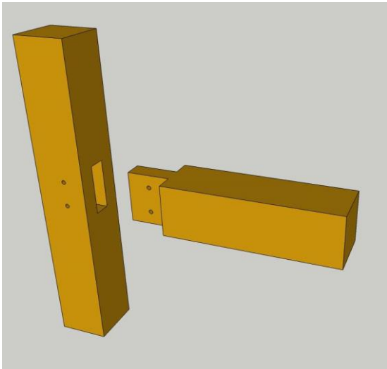
122 Pen-en gatverbinding
