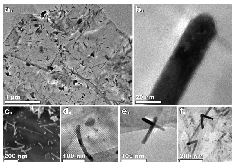
Figure 6. (a) TEM micrograph of a graphene nanoplatform after 10 ALD cycles carried out at 300 °C using the pulsing sequence: 2 min \text{TiCl}_4 —5 min \text{N}_2 —30 s \text{H}_2\text{O} —5 min \text{N}_2 . (b) TEM micrograph of the tip of a NR encapsulated by an amorphous layer. Field emission SEM micrograph of the \text{TiO}_2 /graphene composites obtained after 10 cycles at 300 °C (c) using the same pulsing sequence as in (a). Selection of TEM micrographs of NRs of peculiar morphology: curved NR (d), NR aligned with the edge of the nanoplatform (e), and v-shaped NRs (f).
