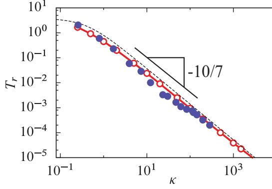
FIG. 3. Film rupture time versus dimensionless meniscus curvature \kappa . The red markers are numerical calculations. The dotted line is the theoretical prediction T_r = 3.92[1 + 3.74\kappa^{10/7}]^{-1} obtained by matching the two self-similar solutions from Fig. 2. The blue markers represent experimental data of rupture times of ethanol films deposited around long bubbles on a PDMS surface.
