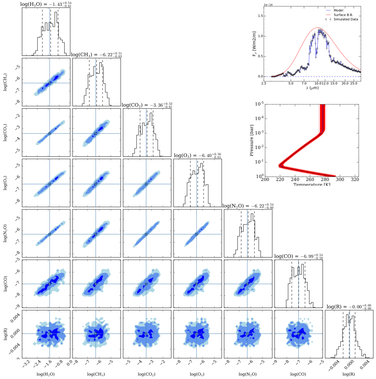
Figure 2: Results of a retrieval study of an Earth-twin atmosphere observed over a wavelength range of 3–30 μm with R = 100 and \text{SNR} = 20 . The inlay in the top right corner shows the model in blue, the simulated observational data in black and a black-body curve representing surface emission in red. Below, the corresponding pressure-temperature profile is plotted with the model again in blue, the best-fit retrieved profile in black and the red band indicating the 68% confidence range. The corner plot shows the marginalized distributions for the abundance of major molecules detected in the atmosphere as well as for the radius of the planet, all of which were free parameters in the retrieval (with flat priors). All parameters are well constrained. We note that also the planet’s mass was a free parameter in the retrieval analysis (with a flat prior confined to the range 0.1–10 M_\oplus ). As expected, it could not be accurately estimated from the spectrum alone and complementary RV measurements or an empirically calibrated mass-radius relationship (e.g., Chen & Kipping, 2017) would be needed to provide constraints.
