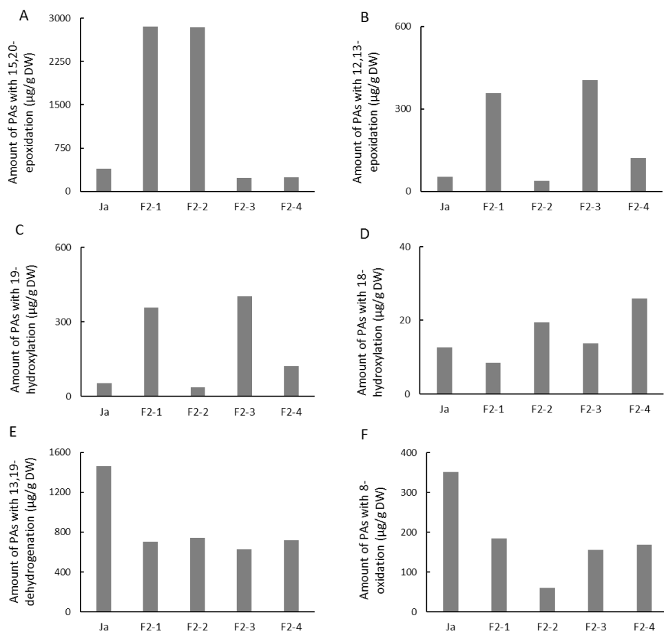
Figure 2. The total concentrations of PAs with the same site-specific oxidative modification derived from the central PA senecionine N -oxide in the shoots of J. aquatica (Ja) and four F 2 groups of a cross between J. vulgaris and J. aquatica . (A) 15,20-epoxidation (including hydrolysis and chlorolysis of 15,20-epoxide); (B) 12,13-epoxidation (including hydrolysis and chlorolysis of 12,13-epoxide); (C) 19-hydroxylation (including acetylation of 19-hydroxyl); (D) 18-hydroxylation; (E) 13,19-dehydrogenation; (F) 8-oxidation. DW: dry weight.
