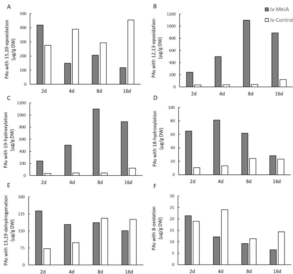
Figure 3. Effects of 90 \mu M MeJA on PA concentrations in the shoots of tissue culture clones of J. vulgaris at different days (d) after treatment. (A) Total amount of PAs with 15,20-epoxidation; (B) total amount of PAs with 12,13-epoxidation; (C) total amount of PAs with 19-hydroxylation; (D) total amount of PAs with or 18-hydroxylation; (E) total amount of PAs with 13,19-dehydrogenation; (F) total amount of PAs with 8-oxidation. DW: dry weight.
