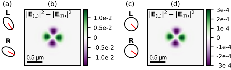
Figure 3.7: Difference in calculated foci for perfectly centred Gaussian beams with elliptical polarizations of opposite handedness. (a) Illustration of the polarization states used in (b); eccentricity \varepsilon = 0.8 , rotated by \pm 30^\circ relative to one another. (b) Difference in intensity distribution between the two. (c, d) Same as (a, b) with parameters closer to the measured polarisation states: \varepsilon = 0.14 , \pm 10^\circ shift.
