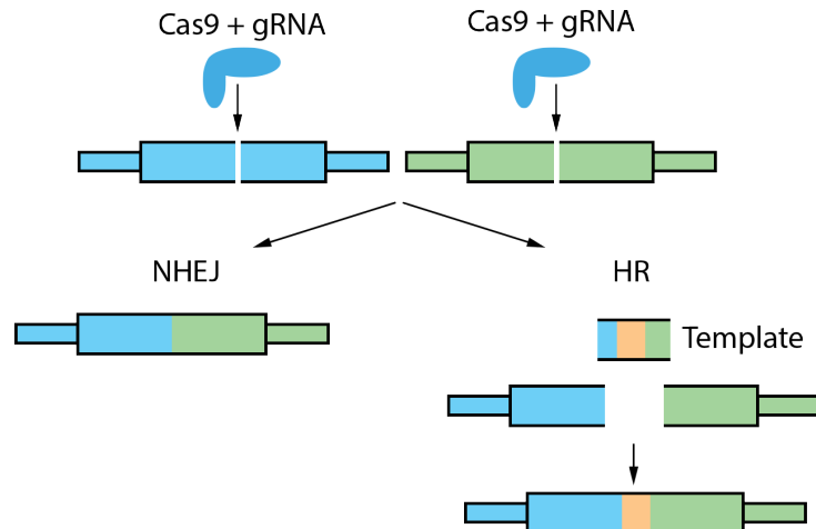
Figure 1.3: Induction of translocations using CRISPR/Cas9. Two break points are introduced and both the NHEJ and HR can lead to the formation of a translocation.
