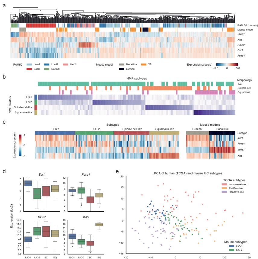
Figure 2 Gene expression analysis of SB-induced tumors. (A) Unsupervised clustering analysis (Euclidean distance, average linkage) of the SB-induced tumors (n = 123) with human breast cancer samples from TCGA (LumA, n = 231; LumB, n = 127; basal-like, n = 95; HER2-enriched, n = 57 and normal-like, n = 29) and tumors derived from mouse models of luminal (n = 20) and basal-like (n = 22) breast cancer using the PAM50 gene signature. The clustering was performed using 46 orthologous mouse genes from the PAM50 signature, but only a representative subset of genes is shown. (B) Coefficient matrix from the non-negative matrix factorization (NMF) analysis of the SB-induced tumors, indicating the membership of each sample to each of the four subtypes (ILC-1, n = 34; ILC-2, n = 33; spindle-cell-like, n = 30; squamous-like, n = 26). The matrix is annotated with the morphological characteristics of samples and shows a clear association between the clusters and the different morphologies. (C-D) Heat map (C) and quantification (D) of the expression of four key genes from the PAM50 gene signature for the different SB-induced subtypes and the mouse reference models, highlighting differences in expression between the different subtypes described in b. SC, spindle-cell-like; SQ, squamous-like. Boxes extend from the third (Q3) to the first (Q1) quartile (interquartile range, IQR), with the line at the median; whiskers extend to Q3 + 1.5 \times IQR and to Q1 - 1.5 \times IQR . Points beyond the ends of the whiskers are outliers. (E) Principal component analysis (PCA) plot comparing the two mILC subtypes to the hILC subtypes from TCGA (immune-related, n = 50; reactive-like, n = 50; proliferative, n = 27) using orthologous genes from TCGA's 60-gene subtype classifier. a.u., arbitrary units.
