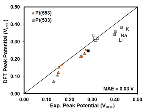
Figure 3.7 DFT-calculated equilibrium potential to exchange 1 ML H^* with OH^* on the step of the Pt(553) surface 13 (triangles) and the Pt(533) surface (squares) plotted against the experimentally measured potential of the sharp, step-associated peak. The solid black square represents the location of the peak measured at low pH (pH 1-3) in the absence of alkali-metal cations, with a simulated hydroxyl coverage of 1/6 ML. The white squares correspond to potentials measured at pH 3 in the presence of 0.01 mol/L Li, Na, K, and Cs and simulated with a hydroxyl coverage of 1/6 ML and Li, Na, K, or Cs coverage of 1/6 ML. The solid gray squares correspond to potentials measured at pH 13 in 0.1 mol/L LiOH, NaOH, and KOH, with a simulated hydroxyl coverage of 1/3 ML and adsorbed Li, Na, and K coverage of 1/3 ML. The solid black line is y = x , and the calculated mean absolute error is 0.03 V.
