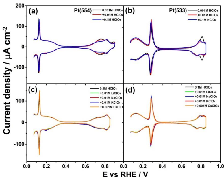
Figure 3.1 Cyclic voltammograms of Pt(554) recorded in (a) 0.1 M \text{HClO}_4 (pH 1), 0.01 M \text{HClO}_4 (pH 2), and 0.001 M \text{HClO}_4 (pH 3), (c) 0.1 M \text{HClO}_4 (pH 1) with 0.01 M \text{LiClO}_4 , \text{NaClO}_4 , and \text{KClO}_4 and 0.001 M \text{CsClO}_4 , and (b, d) the same for Pt(533). Scan rate: 50 \text{ mV s}^{-1} .
