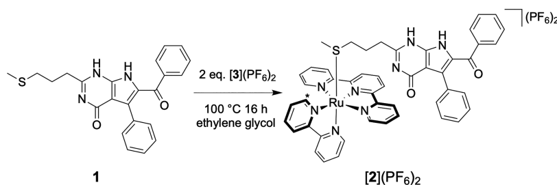
Figure 2. Synthesis of [2](\text{PF}_6)_2 . * indicates the A6 proton of the 2,2'-bipyridine (bpy) ligand.
