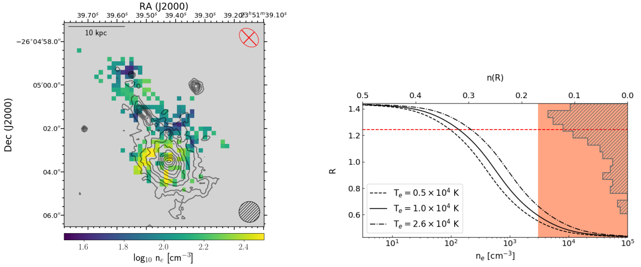
Figure 9. Left panel: Electron density ( n_e ) map for Abell 2667 BCG as retrieved from Eq. 2 for an electron temperature T_e = 1.0 \times 10^4 K, with contours and symbols as defined in Fig. 2. Right panel: Electron density ( n_e ) curve (Proxauf et al. 2014) as a function of the intensity ratio R = [\text{SII}]\lambda 6716/[\text{SII}]\lambda 6731 for T_e = 0.5 \times 10^4 K (black dashed line), T_e = 1.0 \times 10^4 K (black solid line) and T_e = 2.6 \times 10^4 K (black dash-dotted line). The red area of the diagram highlights the electron density values above the [SII] doublet critical density (i.e. n_e \sim 3 \times 10^3 \text{ cm}^{-3} ). We present the distribution of the retrieved R values as well as the median value of the distribution R \sim 1.21 (red dashed line).
