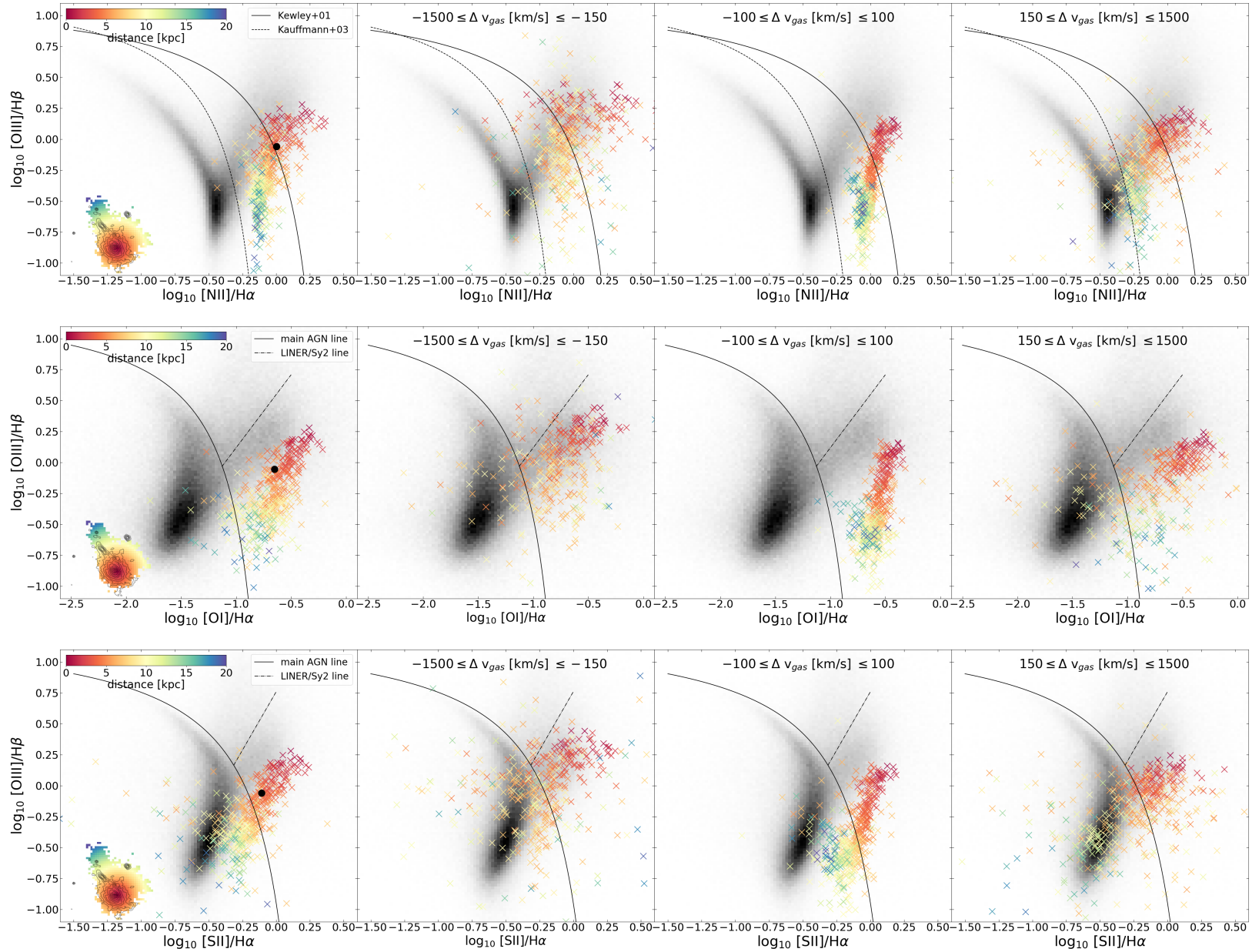
Figure 8. From top to bottom, the BPT-[NII], BPT-[OI] and the BPT-[SII] diagrams for the spaxels with \text{SNR}([\text{OIII}]\lambda 5007) > 3 . For each diagnostic, from left to right we report the diagram obtained integrating all the fluxes within -1500 \text{ km s}^{-1} to 1500 \text{ km s}^{-1} , and in the velocity ranges -1500 \text{ km s}^{-1} to -150 \text{ km s}^{-1} ( blueshifted outflow ), -100 \text{ km s}^{-1} to 100 \text{ km s}^{-1} ( disc ) and 150 \text{ km s}^{-1} to 1500 \text{ km s}^{-1} ( redshifted outflow ), respectively. Each mark is representative of a spaxel and is colour-coded according to its distance from the BCG centre (see the colourbar on the top left and the colour map on the bottom left of the left side panels). To separate the loci corresponding to star-forming galaxies, transition objects and AGNs, we report the empirical relations by Kewley et al. 2001 and Kauffmann et al. 2003. Finally, we report in black the distribution of the emission line galaxies in the Sloan Digital Sky Survey (SDSS) DR7 (Abazajian et al. 2009).
