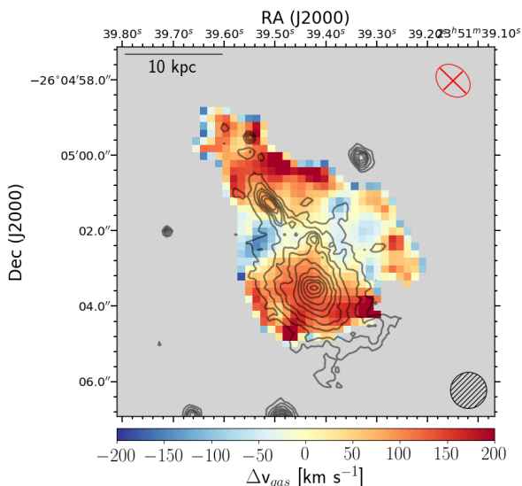
Figure 6. Map of the gas line-of-sight mean velocity ( \Delta v_{gas} ) with respect to the BCG rest-frame, with contours and symbols as defined in Fig. 2. The grey spaxels correspond to spectra with a SNR for the H\beta < 5 .
