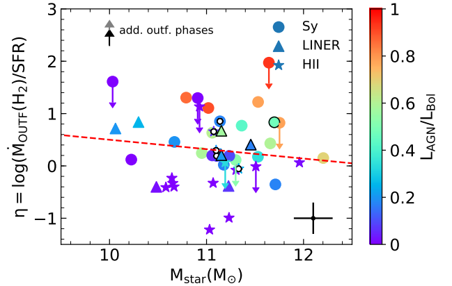
Figure 9. Mass-loading factor as a function of stellar mass. The red dashed line shows the best-fit to the data. Colour-coding and symbols are as in Fig. 1.
