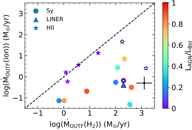
Figure 1. Molecular outflow mass rate ( \dot{M}_{\text{outf}}(\text{H}_2) ) compared to the ionized outflow mass rate ( \dot{M}_{\text{outf}}(\text{ion}) ). The dashed line shows the 1:1 relation. Circles indicate Seyfert host galaxies, LINERs are plotted as triangles and purely star forming galaxies as stars. The data points are colour-coded according to their AGN contribution ( L_{\text{AGN}}/L_{\text{bol}} ), as given in the colour bar on the right. The data points with black edges are molecular outflows inferred from OH measurements by González-Alfonso et al. (2017). The symbols with a central white dot are the candidate “fossil” outflows (see sect.4.3).
