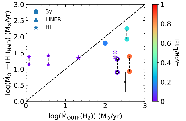
Figure 3. Molecular outflow mass rate ( \dot{M}_{\text{outf}}(\text{H}_2) ) compared to the atomic neutral mass outflow rate inferred from the Na I D absorption ( \dot{M}_{\text{outf}}(\text{HI})_{\text{NaID}} ). The points connected with a dashed line represent two estimates of the neutral outflow rate, one from the literature and one the value re-calculated by us for homogeneity with the rest of the work (see Sect. 2.6). The dashed line shows the 1:1 relation. Colour-coding and symbols are as in Fig. 1.
