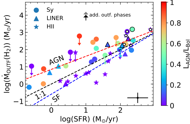
Figure 5. Mass outflow rate as a function of star formation rate. The black dashed line shows the relation for a outflow mass-loading factor \eta = \dot{M}_{\text{outf}}(\text{H}_2)/\text{SFR} = 1 . The black dashed line is the 1:1 relation between outflow rate and SFR, i.e. \eta = 1 . The red and blue dashed lines represent the best fits to AGN hosts and star forming/starburst galaxies, respectively. The vertical black and grey arrows indicate the average correction of the outflow rate, for AGN and star forming galaxies, respectively, once the atomic (ionized and neutral) phases average contributions to the of the outflow rate (as inferred in Sect. 3.1) are included. Colour-coding and symbols are as in Fig. 1.
