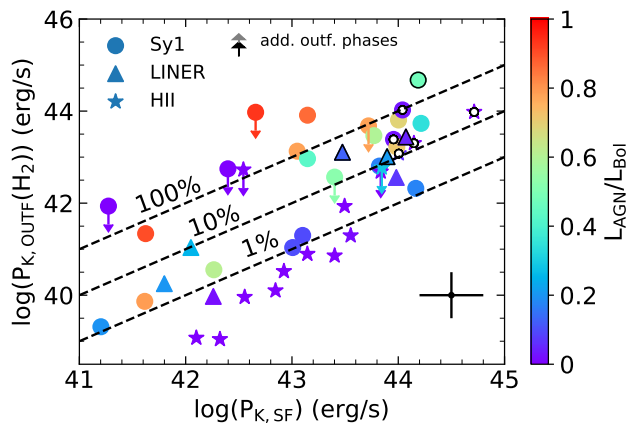
Figure 18. Kinetic power of the outflow as a function of the kinetic power generated by supernovae, as inferred from the SFR. The black dashed lines indicate coupling efficiencies of 1, 10 and 100 per cent. Colour-coding and symbols are as in Fig. 1.
