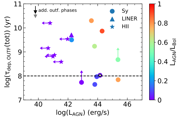
Figure 16. Total gas (HI+H 2 ) depletion time-scale as a function of AGN luminosity. Colour-coding and symbols are as in Fig. 1.
