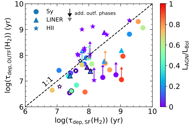
Figure 15. Molecular gas depletion time-scale due to outflows vs depletion time-scale due to star formation. Colour-coding and symbols are as in Fig. 1.
