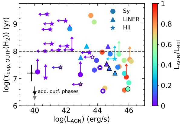
Figure 14. Molecular gas depletion time-scale due to outflows as a function of AGN luminosity. Colour-coding and symbols are as in Fig. 1.
