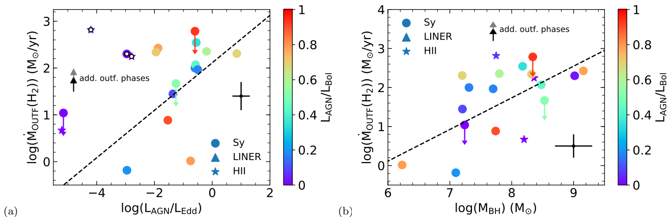
Figure 12. Outflow rate as a function of Eddington ratio, i.e. L_{\text{AGN}}/L_{\text{Edd}} . Outflow rate as a function of black hole mass. Colour-coding and symbols are as in Fig. 1.
