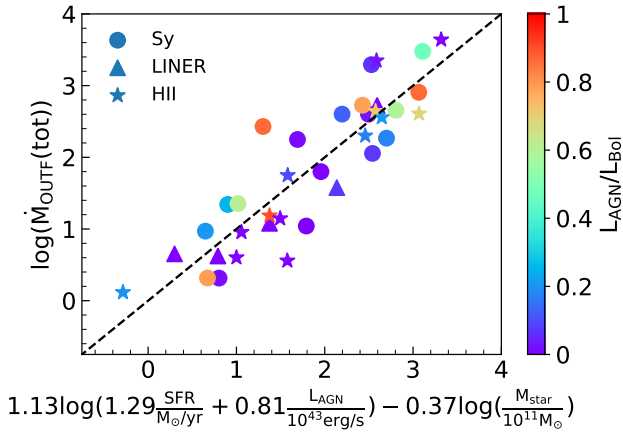
Figure 11. Simultaneous multiple linear regression fit of the total outflow rate as a function of star formation rate, stellar mass and AGN luminosity, as given in equation 6. Colour-coding and symbols are as in Fig. 1.
