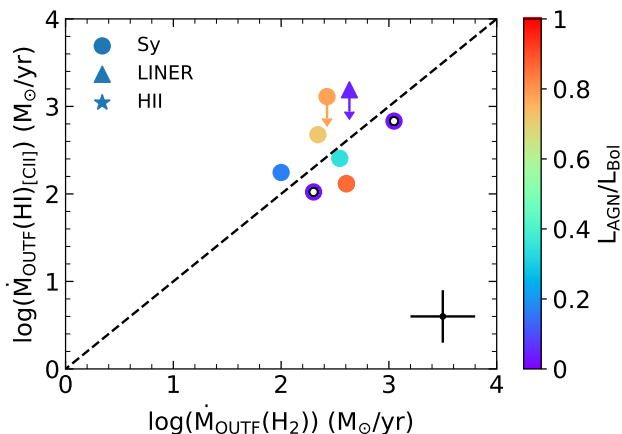
Figure 4. Neutral atomic outflow rates inferred from the [CII] line as a function of the molecular outflow rates. The dashed line gives the 1:1 relation. Colour-coding and symbols are as in Fig. 1.
