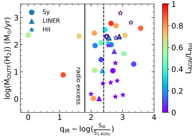
Figure 13. Molecular outflow rate as a function of the parameter q_{\text{IR}} defined as the ratio between the far-IR flux and the radio monochromatic flux at 1.4 GHz (Sect.2.4.6). The vertical dashed line indicates the average value for star forming galaxies, while the solid vertical line indicates the limit below which galaxies are considered to have a significant radio excess associated with a radio jet (Ivison et al. 2010; Harrison et al. 2014). Colour-coding and symbols are as in Fig. 1.
