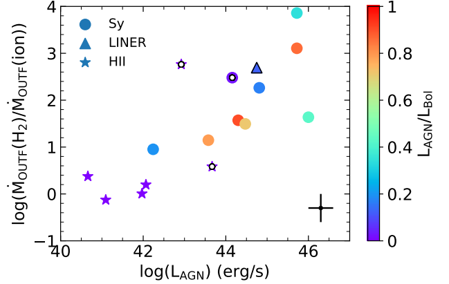
Figure 2. Molecular to ionized mass outflow rate as a function of AGN luminosity. Colour-coding and symbols are as in Fig. 5.
