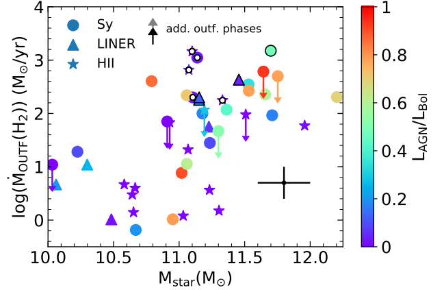
Figure 8. Molecular outflow mass rate as a function of galaxy stellar mass. Colour-coding and symbols are as in Fig. 1.
