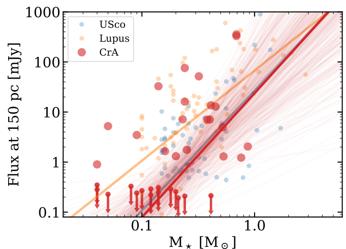
Fig. 5: Correlation between dust disk flux scaled at 330 GHz (assuming \alpha = 2.25 , as in Ansdell et al. 2018) and at a distance of 150 pc with stellar mass for the objects in CrA. The slopes of Lupus and Upper Sco are also plotted for comparison. We show the results of the Bayesian fitting procedure by Kelly (2007). The solid line represents the best fit model, while the light lines show a subsample of models from the chains, giving an idea of the uncertainties.
