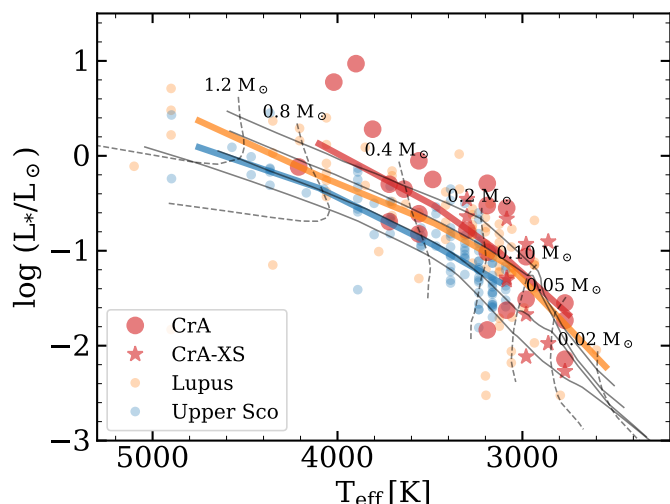
Fig. 6: HR diagram showing the sources in our CrA sample (red), in the Lupus sample from Ansdell et al. (2016) (orange) and in the Upper Sco sample (blue) from Barenfeld et al. (2016). The evolutionary tracks for different stellar masses and the relative isochrones from Baraffe et al. (2015) are also plotted for reference. The isochrones refer (from top to bottom) to the 1 Myr, 2 Myr, 5 Myr and 10 Myr isochrone. The coloured solid lines show the approximate median value of the luminosity at each temperature.
