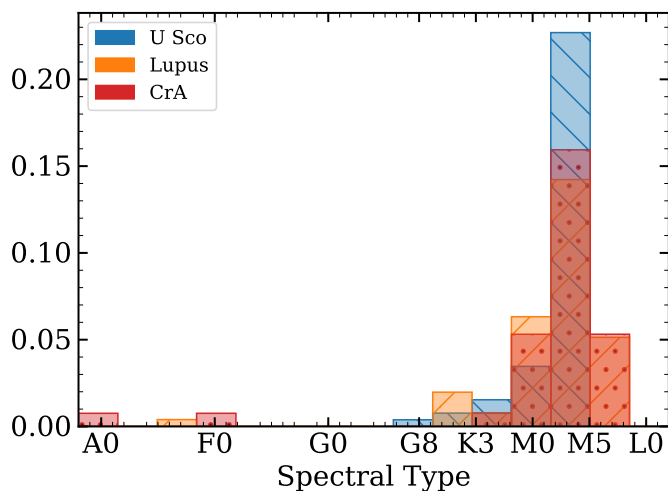
Fig. 2: Distribution of the spectral types of the stars in CrA (Red) compared to that of Lupus (Orange) and Upper Sco (Blue).
