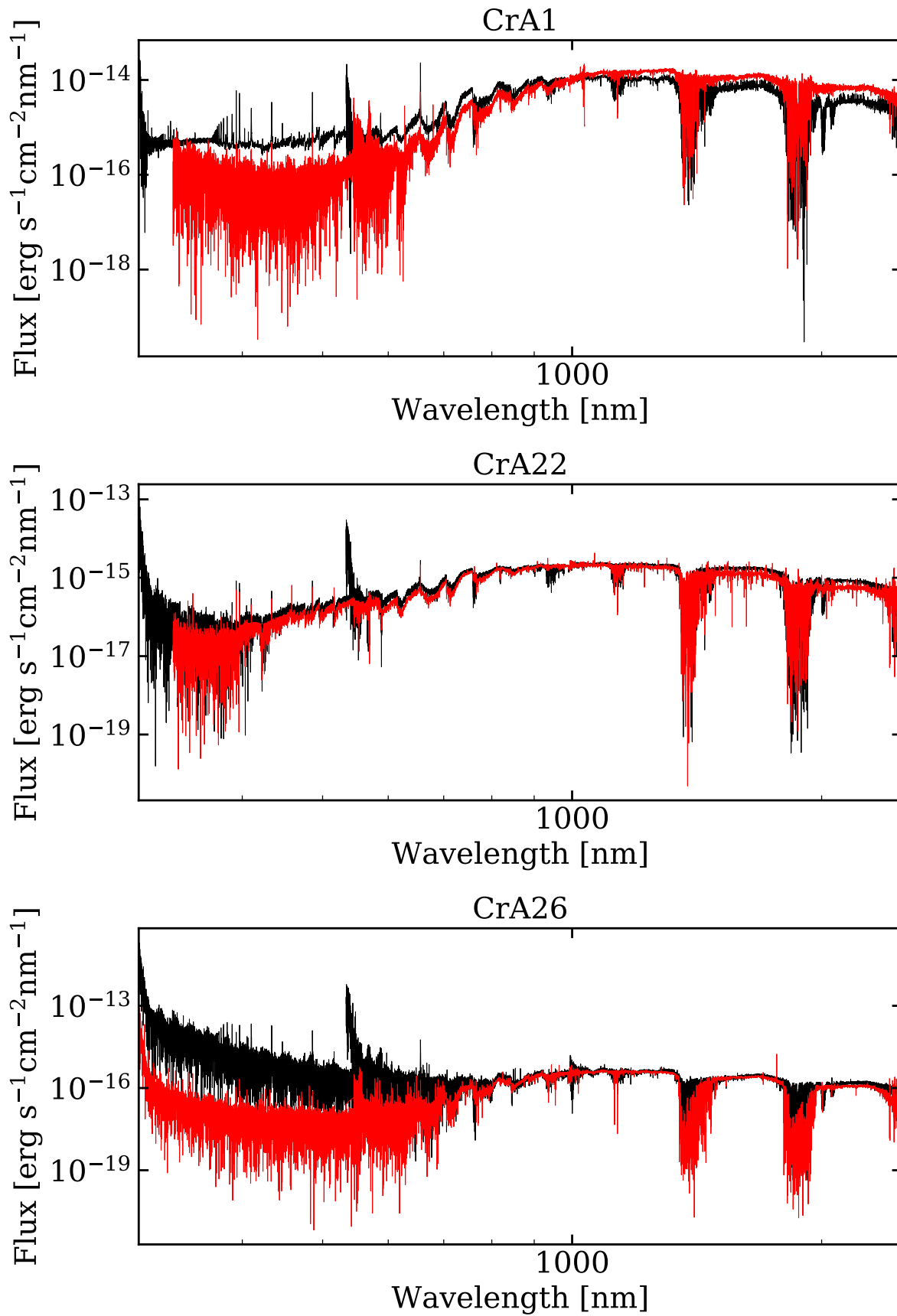
Fig. B.1: Spectra observed in our X-Shooter programs (black) along with a template with the same Spectral Type (red). The name of the sources is in the title of each subfigure. The absolute flux of each template was normalized to the flux of the observation at \lambda = 1\mu\text{m} .
