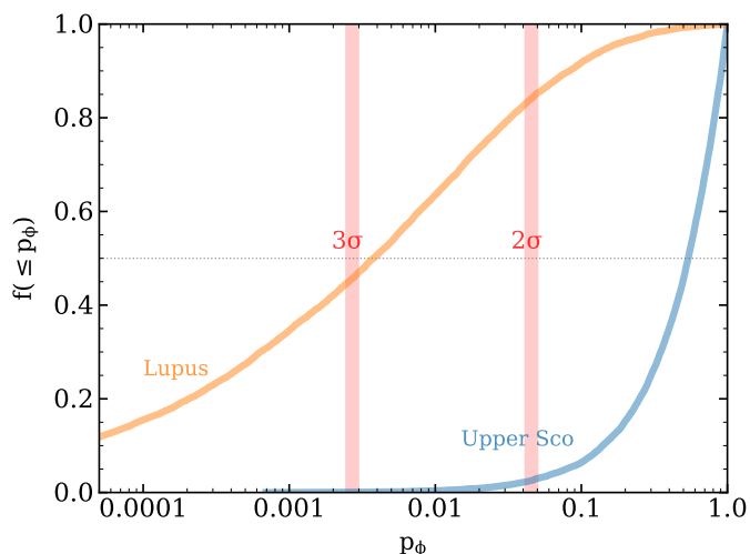
Fig. 7: Comparison of the mass distributions of Lupus and USco to that of CrA, following the MC analysis proposed by Andrews et al. (2013). p_\phi is the probability that the synthetic population drawn from the comparison sample (Lupus and Upper Sco) and the reference sample come from the same parent population. f(< p_\phi) is the cumulative distribution for p_\phi resulting from the logrank two-sample test for censored datasets after 10^4 MC iterations.
