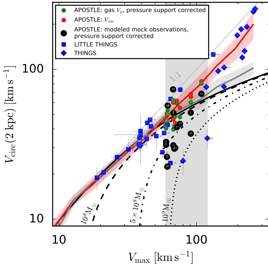
Figure 9. Circular velocity at 2 kpc plotted against maximum circular velocity, a measure of the ‘central mass deficit’. The lines are reproduced from fig. 6 of Oman et al. (2015, see their sec. 4.6 for additional details). The solid black line indicates the expected correlation for an NFW (Navarro et al. 1996b, 1997) mass profile and the mass concentration relation of Ludlow et al. (2014); this is well traced by haloes in dark-matter-only versions of the APOSTLE and EAGLE simulations. Values measured from the circular velocity profiles of galaxies from the (hydrodynamical) APOSTLE and EAGLE simulations lie along the red line. The broken lines indicate the correlation for the same (NFW) profile but removing a fixed amount of mass from the central 2 kpc, as labelled. Three points are shown for each of the APOSTLE galaxies in our sample: one for the circular velocity at 2 kpc (red), another for the gas azimuthal speed corrected for pressure support (green), and a third for the 3^{\text{D}} BAROLO estimates of the rotation speed corrected for pressure support (black). Each quantity is shown as a function of the maximum of the circular velocity of each system, V_{\text{max}} . Galaxies that we have flagged as kinematically disturbed (see Fig. 4 and Sec. 5.1) are omitted. The grey shaded area marks our selection in V_{\text{max}} , as in Fig. 1. We show measurements from the THINGS (blue diamonds) and LITTLE THINGS (blue squares) surveys for comparison.
