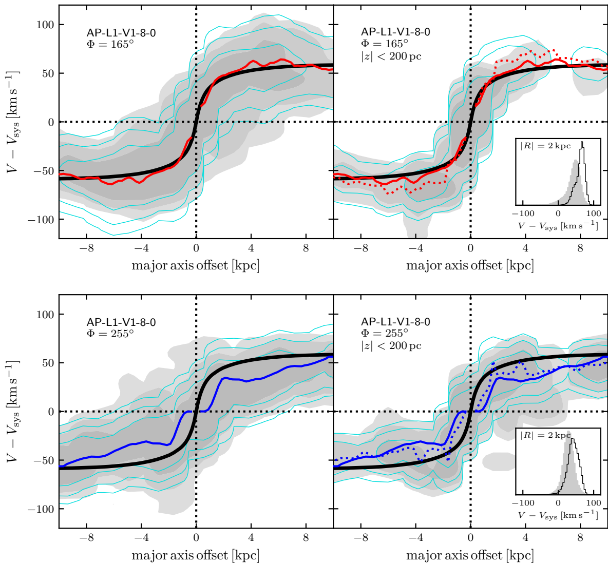
Figure 10. Left panels: Position-velocity (PV) diagrams along the major axis for two projections of AP-L1-V1-8-0 offset by 90^\circ : \Phi = 165^\circ (top row) and \Phi = 255^\circ (bottom row). The synthetically observed data for a \sim 500 pc (30 arcsec) wide slice along the major axis is shown with filled contours; the levels are drawn at signal-to-noise levels of 0.3, 3 and 30, assuming a fiducial noise level of 0.4 \text{ mJy beam}^{-1} , similar to that of the THINGS survey (Walter et al. 2008). The open contours correspond to the same slice through the model data cube produced by 3\text{D BAROLO} , with the contours drawn at the same levels. The coloured curve shows the 3\text{D BAROLO} -derived rotation curve, and the black curve shows the spherically-averaged circular velocity profile. Right panels: Similar to the left panels, except that the synthetic observations have been made considering only those gas particles within 200 pc of the galactic mid-plane. The contour levels have been shifted 1-dex fainter to make the distribution visible. The coloured solid lines reproduce the rotation curves from the left panels, while the dotted lines show the rotation curve fit for the mid-plane gas. Inset panels: Normalized histograms showing the velocity distributions along the major axis at R = 2 kpc in the synthetic data cubes, i.e. a ‘vertical’ slice through the distributions shown with filled contours in the PV diagrams. The filled histogram corresponds to the entire gas distribution, the open histogram to only the gas within 200 pc of the midplane.
