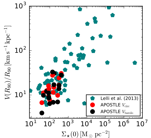
Figure 15. Central rotation curve slope, which we parametrize as V(R_{90})/R_{90} , as a function of central stellar surface density, \Sigma_{\star}(0) ; R_{90} is the radius where the circular velocity curve reaches 90 per cent of its maximum amplitude. For our sample of ‘equilibrium’ APOSTLE galaxies, we show both the central rotation curve slope as measured from the circular velocity curve (red points), and from the rotation curve derived using 3D BAROLO (black points). We show for comparison measurements from Lelli et al. (2013, pentagons). We have converted their central surface brightnesses to central surface densities assuming a mass-to-light ratio in the R -band of \Upsilon_R^{\star} = 3.0 M_{\odot} L_{\odot}^{-1} , and a Solar magnitude of 4.5 in the R -band.
