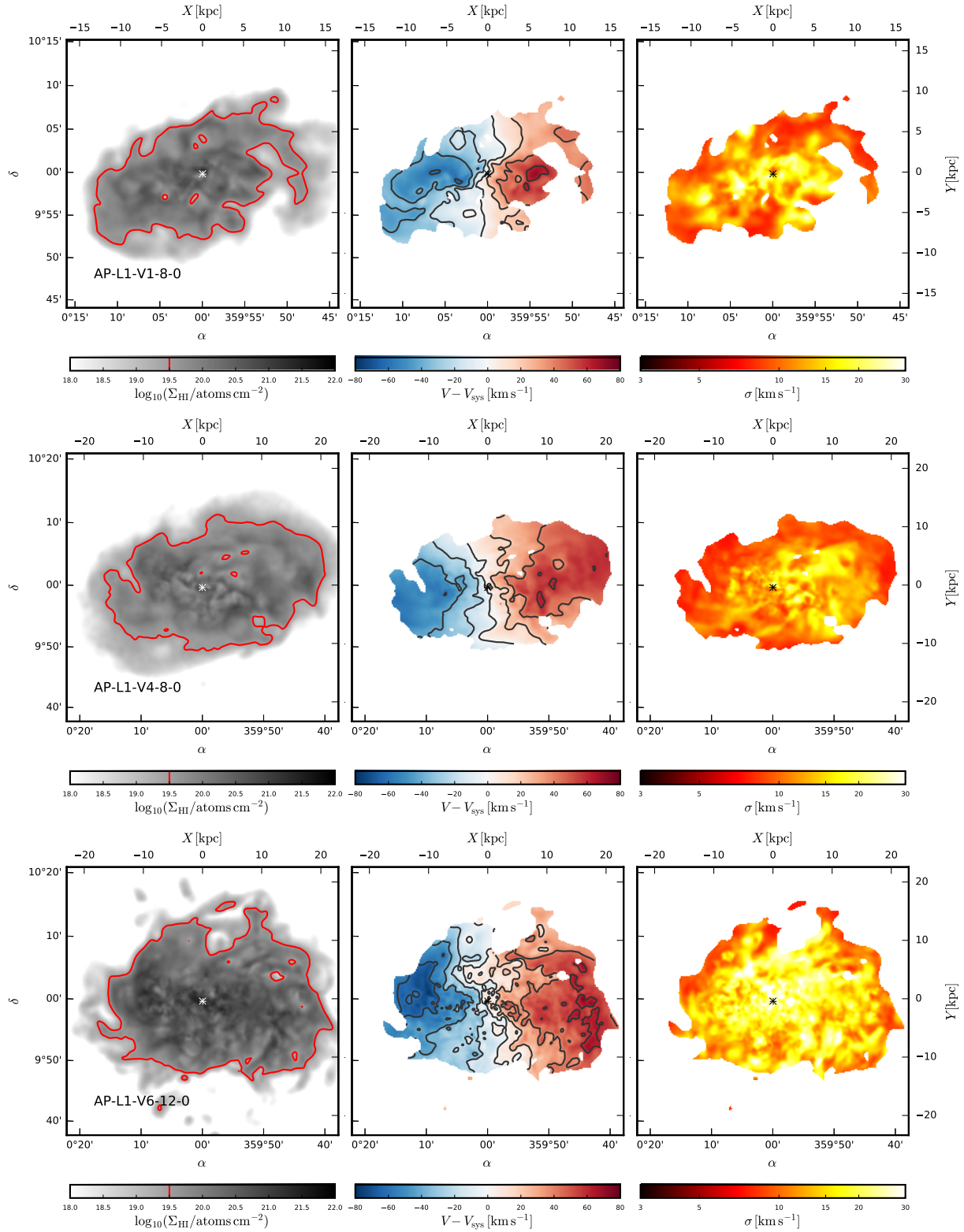
Figure 2. From left to right: 0 th moment (surface density), 1 st moment (flux-weighted mean velocity) and 2 nd moment (flux-weighted velocity dispersion) maps for three objects in our sample of APOSTLE galaxies. The galaxies are placed at an arbitrary sky position at a distance of 3.7 Mpc, inclination of 60° and position angle of 270° (angle East of North to the approaching side), where the angular momentum vector of the H I disc is taken as the reference direction. The 1 st and 2 nd moment maps are masked to show only pixels where the surface density exceeds 10^{19.5} atoms \text{cm}^{-2} (indicated by the red line in the surface density map). Contours on the 1 st moment map correspond to the tick locations on the colour bar. The ‘×’ marks the location of the potential minimum, which is well-traced by the peak of the stellar distribution, marked ‘+’. See also Appendix E.
