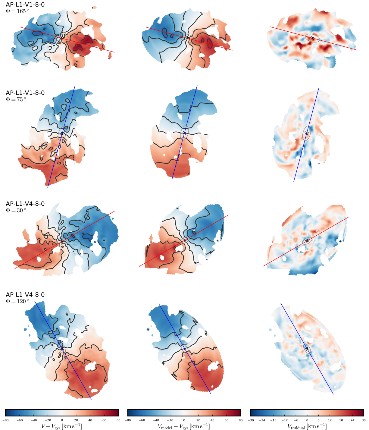
Figure 8. Left column: Velocity maps for the same two galaxies shown in Figs. 5–7 along lines of sight which place the red (rows 1 & 3, rotation curve systematically overestimated) or blue (rows 2 & 4, rotation curve systematically underestimated) lines from the upper panels of Fig. 6 along the major axis. The grey ellipse marks R = 2 kpc; the isovelocity contours are drawn at the same positions as the tick marks on the colour bars. Centre column: Velocity maps extracted from the 3^{\text{D}} BAROLO model data cubes for the same galaxies and orientations. Right column: Difference of the left and centre columns (note that the colour scale is compressed).
