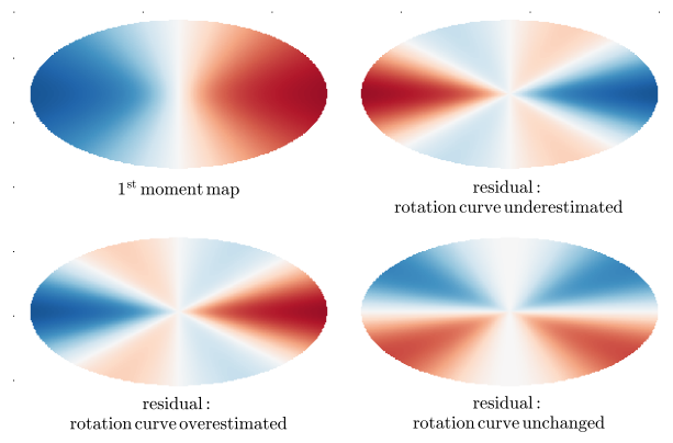
Figure C2. Given a rotating disc oriented as illustrated in the upper left panel, an azimuthal m = 2 modulation of the velocity field whose orientation is such that it causes an underestimate of the rotation curve (minima along the line of nodes) results in a three-peaked residual pattern, illustrated in the upper right panel. Note the residual peak (red in upper right) lying on the approaching side of the disc (blue in upper left). The case corresponding to an overestimate of the rotation curve (maxima along the line of nodes) is illustrated in the lower left panel; the residual is reflected relative to the case of an underestimate. In the case where the m = 2 pattern causes no change to the rotation curve estimate (lower right), the residual is null along the line of nodes.
