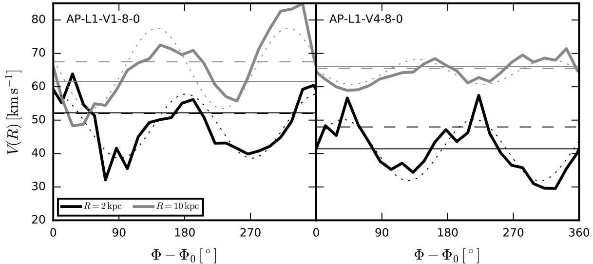
Figure 7. Rotation velocity at 2 and 10 kpc as recovered by {}^3\text{D} BAROLO as a function of projection axis \Phi , including pressure support corrections. The reference direction \Phi_0 is defined as the nominal direction of the maximum of the m = 2 pattern in the upper quadrants, i.e. the red line in the upper panels of Fig. 6. \Phi_0 = 165^\circ and 30^\circ for AP-L1-V1-8-0 and AP-L1-V4-8-0, respectively. The horizontal dashed lines show the circular velocity at the same radii, while the horizontal solid lines shows the mean rotation velocity of the H I gas, also at the same radii, measured directly from the simulation particles, and corrected for pressure support. We expect the fit rotation speed to vary proportionally to \cos(2(\Phi - \Phi_0)) ; we show the best-fitting V_0 + V_2 \cos(2(\Phi - \Phi_0) - \Phi') with a dotted line (note the additional freedom \Phi' in the phase). In general \Phi' \neq 0 because in some cases the m = 2 pattern (Fig. 6 upper panels) is, at some radii, not exactly aligned along the direction defined by \Phi_0 .
