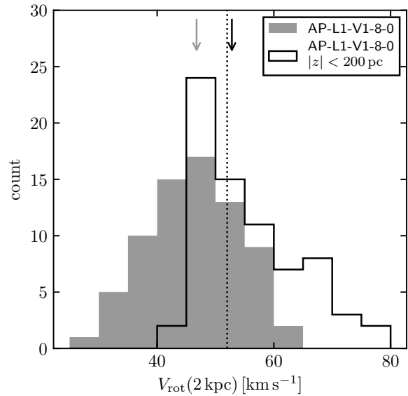
Figure 11. Distribution of H I rotation velocity at R = 2 kpc as recovered using 3^{\text{D}} BAROLO for AP-L1-V1-8-0 for 72 orientations, all at i = 60^\circ , each separated in viewing angle by 5^\circ in azimuth. The filled histogram corresponds to synthetic data cubes constructed using the entire H I gas distribution, whereas for the open histogram, data cubes where any gas more than 200 pc from the galactic mid-plane has been discarded were used instead. The medians of the two distributions are marked with the arrows of corresponding colour, and the circular velocity at 2 kpc is marked by the vertical dotted line.
