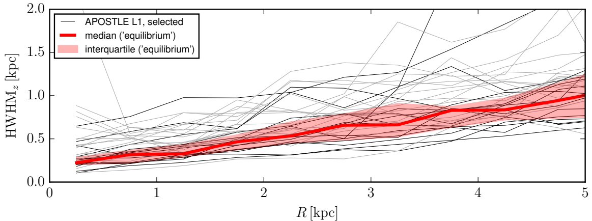
Figure 12. Height enclosing half the mass in H I as a function of radius for APOSTLE galaxies in our sample (thin lines). Our ‘equilibrium’ (‘non-equilibrium’) subsample is shown with black (grey) lines. ‘Equilibrium’ galaxies tend to be slightly thinner, on average. The median and interquartile interval of the distribution of ‘equilibrium’ galaxies are shown by the heavy red line and shaded area, respectively.
