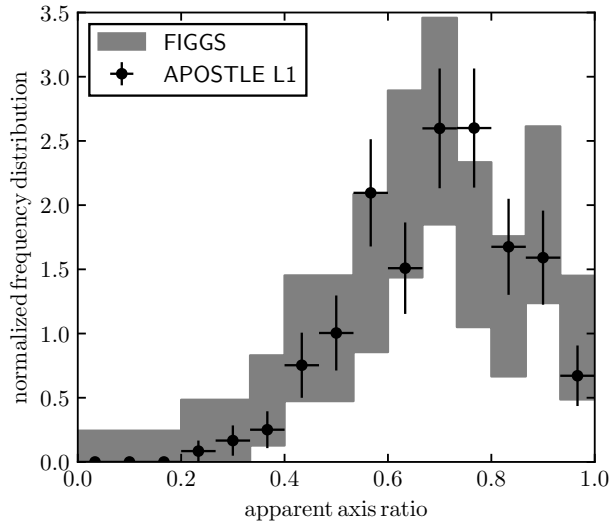
Figure 14. Distribution of apparent beam-corrected axis ratios of the H I distribution in APOSTLE galaxies (points with error bars) at a column density of 10^{19} \text{ cm}^{-2} . The sample is drawn from \sim 200 APOSTLE dwarfs with 20 < V_{\text{max}}/\text{km s}^{-1} < 120 and is constructed to approximately match the median and width of the H I mass distribution of the FIGGS sample of Roychowdhury et al. (2010, see also Begum et al. 2008), whose measurement is reproduced here (grey band). Each APOSTLE galaxy is viewed from a random angle and convolved with a 1 kpc (FWHM) beam, similar to the 44 arcsec beam used to observe the FIGGS sample, at the median distance of 5 Mpc of those galaxies. The vertical error bars/shaded areas represent the Poisson errors on the measurements; the horizontal error bars/shaded areas are the bin widths.
