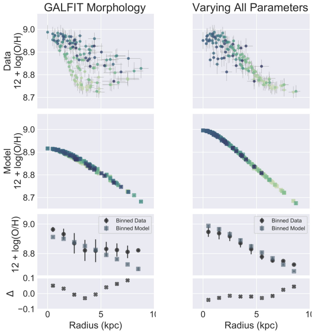
Figure 7. AS1063-arc radial variation of metallicity using the morphology derived from HST with GALFIT (left panels) and letting the morphological parameters free (right panels). Data is shown in the top panels and the model gradient convolved with the seeing is shown in the middle panel. Each point corresponds to a Voronoi bin, colour coded by the number of the bin, so that the same bin has the same colour in all plots and adjacent bins have similar colours. The lower panels display the binned version of both the data (circles) and the model (squares) and the binned residuals (crosses).
