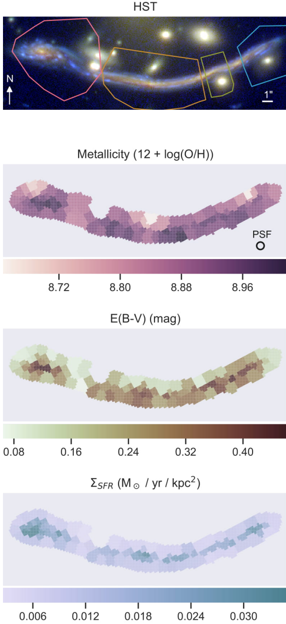
Figure 4. A370-sys1 in the image plane. Top panel: HST composite image with filters F160W, F814W and F435W. Contours correspond to the different multiple images, with the complete image in pink. Lower panels: metallicity, extinction and SFR surface density maps, from top to bottom, each colour coded in a different colour scheme. The FWHM of the PSF plotted in the lower-right corner of the bottom panel. All images have the same physical size and orientation.
