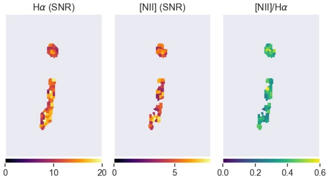
Figure A3. M1206-sys1 signal-to-noise ratios maps of H\alpha and [N\text{II}]\lambda 6585 (left and middle panels) and ratio of the two (right panel).
