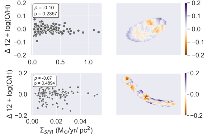
Figure 10. Metallicity gradient residuals. Top: AS1063-arc. Bottom: A370-sys1. Left: residuals after subtracting fitted gradient vs star formation rate density. The Spearman rank-order correlation coefficient and respective p value calculated for each of the two properties plotted are shown in the top-left corner of each plot. Right: 2D residuals map.
