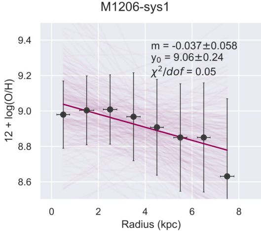
Figure 9. M1206-sys1 radial variation of metallicity. The data points correspond to averages within annuli. The fit was performed with the LINMIX package. The pink lines are multiple realisations of the fit. The thick line corresponds to the average of all these possible slopes, and we plot its slope ( m ) and intercept ( y_0 ) and uncertainties in the top-right corner.
