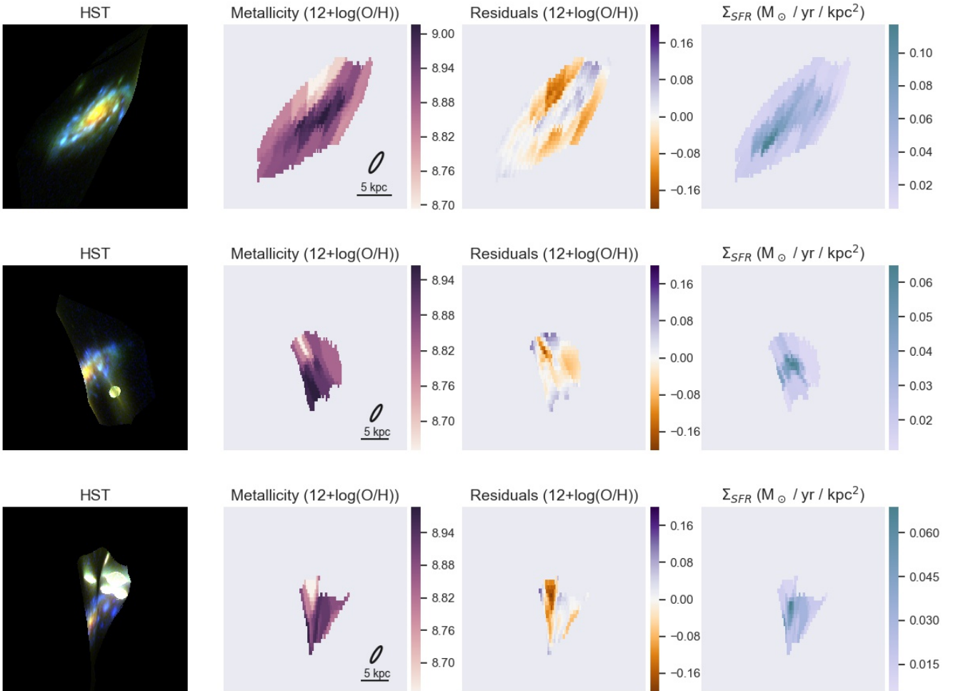
Figure C1. AS1063 in the source plane. Left: HST composite image with filters F160W, F814W and F435W. Middle Left: reconstructed metallicity map. The FWHM of the PSF in the source plane is plotted in the lower-left corner. Middle-right: source plane metallicity residuals, after subtracting the model fitted with all parameters free to vary. Right: SFR surface density map. SFRs were derived from H \beta and the Kennicutt (1998) calibration.
