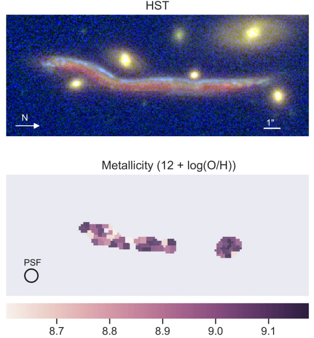
Figure 5. M1206-sys1 in the image plane. Top panel: HST composite image with filters F160W, F814W and F435W. Bottom panel: metallicity derived from \text{H}\alpha and [\text{N II}] \lambda 6585 . The FWHM of the PSF is plotted in the lower-left corner of the bottom panel.
