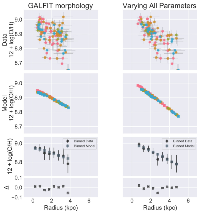
Figure 8. As Fig. 7 but for A370-sys1.
