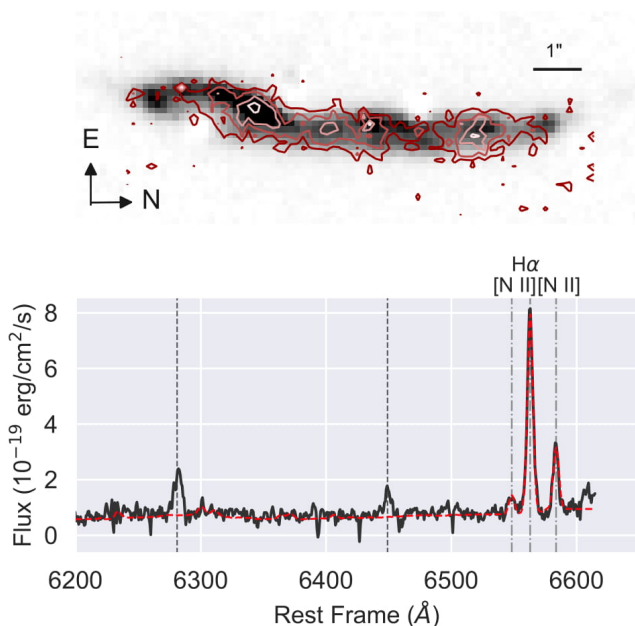
Figure 1. M1206-sys1 data. Top: MUSE [O II] \lambda 3727,29 pseudo-narrow band in grey scale with SINFONI H \alpha pseudo-narrow band image over-plotted in red contours (surface brightness of 2, 3, 4, 5 \times 10^{-19} erg/cm ^2 /s/arcsec ^2 ). Both have been continuum subtracted. Bottom: SINFONI integrated spectrum in black and fit performed with the line fitting code ALFA ( Wesson 2016 ) in dashed red, with the [N II] doublet and H \alpha identified with dashed-dotted lines and strong sky residuals in dashed lines.
