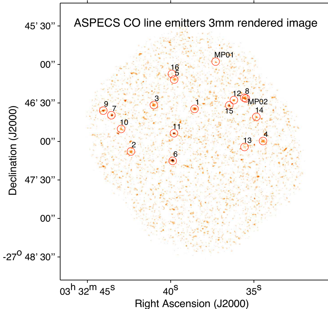
Figure 1. Rendered CO image toward the HUDF, obtained by co-adding the individual average CO line maps around the 16 bright CO-selected galaxies and the 2 lower significance MUSE-based CO sources (labeled MP). Regions with significances below 2.5\sigma in each of the average maps are masked out prior to combination. The location of these individual detections is highlighted by solid circles and their IDs. The tendency of sources to lie in the top two-thirds of the map is likely a combination of clustering and chance, given the sensitivity of the observations is fairly uniform across this region.
