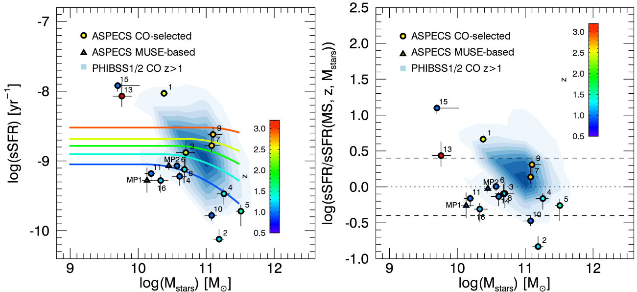
Figure 6. ( Left: ) Specific SFR vs stellar mass diagram for the ASPECS CO sources, compared to z > 1 PHIBSS2 CO sources. ( Right: ) Specific SFR (normalized by the value of the sSFR expected for the MS, which is a function of the redshift and stellar mass) vs stellar mass diagram for the ASPECS CO sources, compared to z > 1 PHIBSS2 CO sources. In both panels, the PHIBSS2 galaxies are represented by the blue contours. In the left panel, the solid lines represent the observational relationships between SFR (or sSFR) and stellar mass at different redshifts derived by Schreiber et al. (2015). These redshifts are denoted in different colors as shown by the color bar to the right. In the right panel, the dotted line represents the location of the MS, while the dashed lines represent the location of sources at +0.4 and -0.4 dex from the MS. Two of the ASPECS CO selected galaxies lie > 0.4 dex below the MS at their respective redshift (3mm.2 and 3mm.10).
