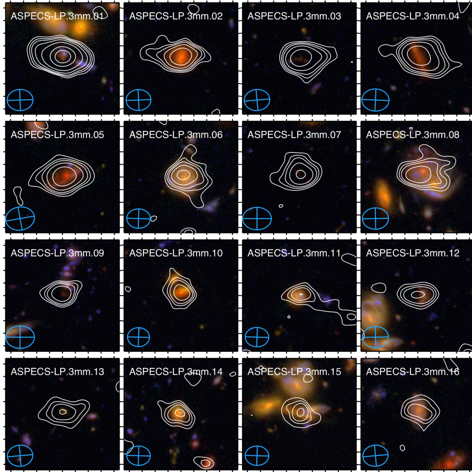
Figure 14. Optical/near-IR postage stamps compared to the CO emission for the ASPECS CO-selected sample. HST RGB images (F435W, F850LP, F105W) are shown in the background with white contours overlaid representing the CO line emission at significances 2, 3, 4, 6, 10, 20 and 30 \sigma , where \sigma is the rms noise level of each CO moment-0 image.
