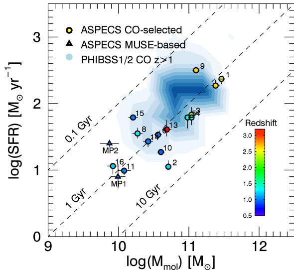
Figure 7. SFR vs. M_{\text{mol}} for the ASPECS CO galaxies compared to the z > 1 PHIBSS2 galaxies (Tacconi et al. 2018), represented by blue contours as in Fig. 5. The dashed lines represent curves of constant t_{\text{dep}} at 0.1, 1 and 10 Gyr. A fixed conversion factor \alpha_{\text{CO}} = 3.6 \text{ (K km s}^{-1} \text{ pc}^2)^{-1} has been assumed for the ASPECS CO sources. The comparison sample uses a metallicity-based prescription for this parameter. Typical values will range between \alpha_{\text{CO}} = 2 - 5 \text{ (K km s}^{-1} \text{ pc}^2)^{-1} for the ASPECS CO sources.
