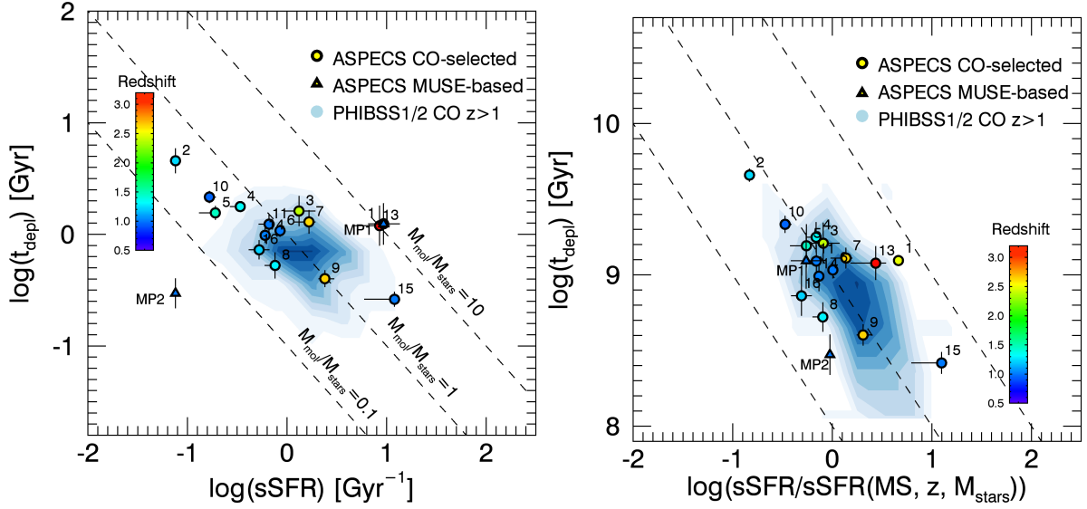
Figure 9. The molecular gas depletion timescale ( t_{\text{dep}} ) as a function of the specific SFR for the ASPECS CO galaxies. In both panels, the background blue contour levels represent the distribution of z > 1 PHIBSS2 CO galaxies, and the coloring of each ASPECS source represents their respective redshift. The left panel shows t_{\text{dep}} as a function of sSFR. Here the dashed lines represent curves of fixed gas fraction ( M_{\text{mol}}/M_{\text{stars}} ). The right panel shows the sSFR normalized by the value of the sSFR expected for the MS (which is a function of the redshift and stellar mass) from Schreiber et al. (2015) . In this case, the dashed lines are shown only for visualization purposes. A fixed conversion factor \alpha_{\text{CO}} = 3.6 \text{ (K km s}^{-1} \text{ pc}^2)^{-1} has been assumed for the ASPECS CO sources. The comparison sample uses a metallicity-based prescription for this parameter. Typical values will range between \alpha_{\text{CO}} = 2 - 5 M_{\odot} \text{ (K km s}^{-1} \text{ pc}^2)^{-1} for the ASPECS CO sources.
