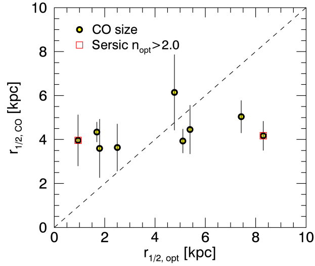
Figure 13. Comparison between the rest-frame optical sizes derived by van der Wel et al. (2012) and the CO sizes measured from the ASPECS data. Only resolved sources in CO emission are considered. Red squares highlight sources for which the optical morphology indicates large Sersic indexes, which would indicate highly concentrated optical emission and thus might not be directly comparable to the CO estimates.
