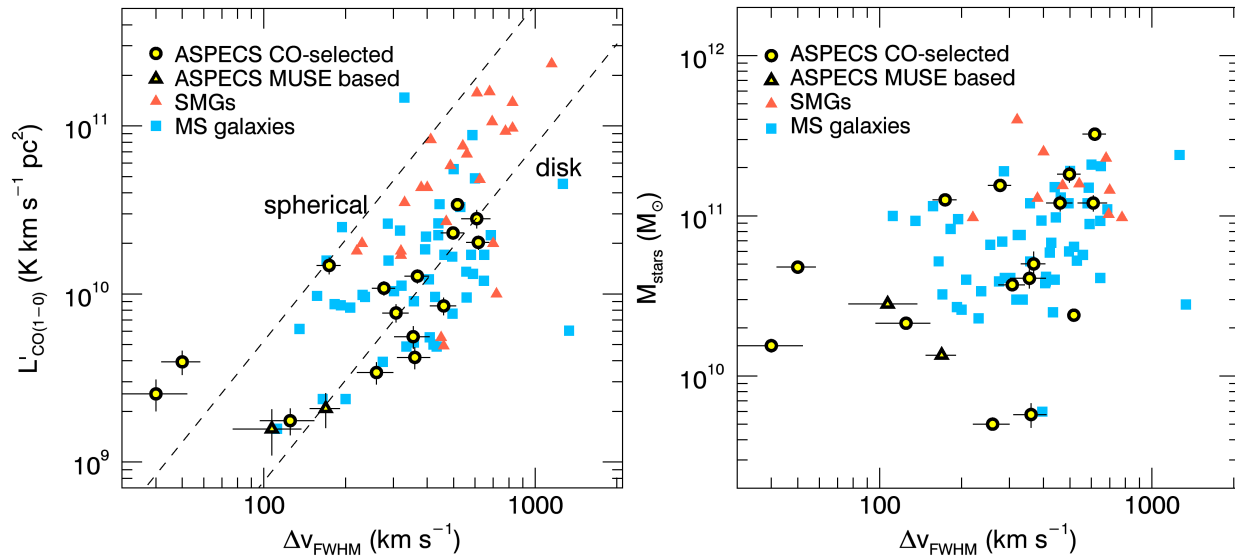
Figure 3. ( Left: ) Estimated CO(1-0) line luminosities as a function of the line widths ( \Delta v_{\text{FWHM}} ) for the ASPECS sources, compared to a compilation of galaxies from the literature detected in CO line emission, including unlensed submillimeter galaxies (Frayser et al. 2008; Coppin et al. 2010; Riechers et al. 2011, 2014; Ivison et al. 2013, 2011; Thomson et al. 2012; Carilli et al. 2011; Hodge et al. 2013; Bothwell et al. 2013; De Breuck et al. 2014) and z > 1 MS galaxies (Daddi et al. 2010b; Magnelli et al. 2012; Magdis et al. 2012; Tacconi et al. 2013; Magdis et al. 2017). The dashed lines represent a simple “virial” functional form for the CO luminosity for a compact starburst and an extended disk (Sect. 3.2). The actual location of each of these lines depend on the choice of geometry and \alpha_{\text{CO}} factor. ( Right: ) Stellar masses versus line widths for the ASPECS sources, compared to literature (where stellar mass estimates are available).
