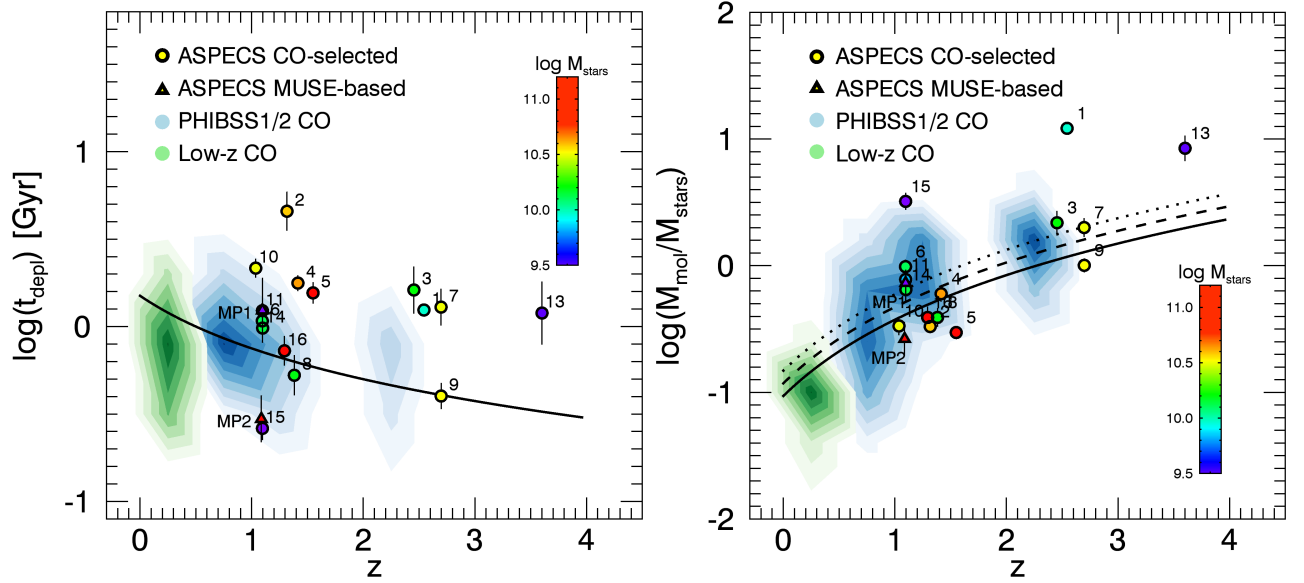
Figure 10. Evolution of the t_{\text{depl}} and f_{\text{mol}} = M_{\text{mol}}/M_{\text{stars}} with redshift. The background blue contour levels represent the distribution of galaxies from the PHIBSS2 compilation. As a reference in redshift, we also show as green contours the distribution of galaxies detected in CO line emission at z < 0.5 from the PHIBSS2 compilation (e.g. from xCOLDGASS, GOALS and EgNOG surveys). The solid lines show the expected evolution of t_{\text{depl}} and f_{\text{mol}} with redshift, based on previous targeted observations of star forming galaxies. A fixed conversion factor \alpha_{\text{CO}} = 3.6 \text{ (K km s}^{-1} \text{ pc}^2)^{-1} has been assumed for the ASPECS CO sources. The comparison sample uses a metallicity-based prescription for this parameter. Typical values will range between \alpha_{\text{CO}} = 2 - 5 M_{\odot} \text{ (K km s}^{-1} \text{ pc}^2)^{-1} for the ASPECS CO sources.
