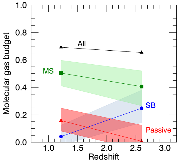
Figure 11. Contribution to the total molecular gas budget from galaxies above (starburst), in or below (passive) the MS as a function of redshift inferred from the ASPECS survey. The blue, green and red data points and lines represent galaxies above, in and below the MS, respectively. The black curve shows the contribution of all the CO-selected galaxies considered here to the total molecular gas at each redshift. Each data point is computed from the sum of molecular gas masses of all galaxies in that redshift bin and galaxy type. The redshift measurement of each point is computed as the average redshift from all galaxies in that bin. The shaded region corresponds to the uncertainties of each measurement.
