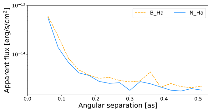
Fig. 12. Apparent flux detection limits as a function of the angular separation from HD142527 for both B_Ha and N_Ha filters. In this specific case, using B_Ha does not help detecting fainter objects in the background limited regime.
