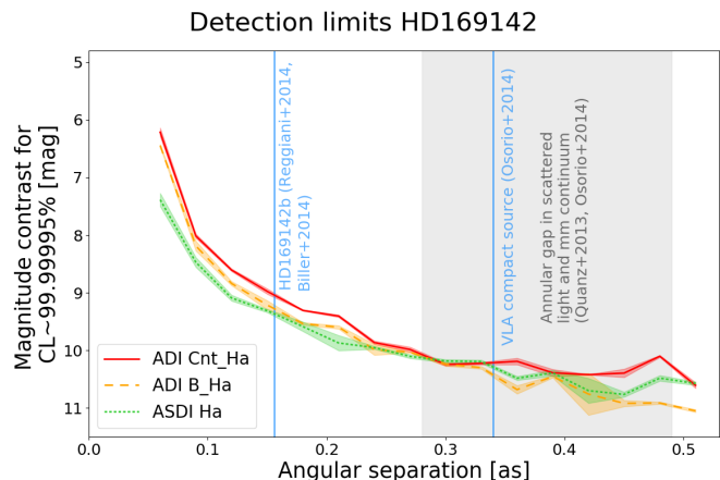
Fig. 9. Contrast curves for HD169142. The shaded region represents the annular gap observed in scattered light (Quanz et al. 2013b) and in mm-continuum (Osorio et al. 2014). The blue vertical lines represent the separation of the companion candidates (Reggiani et al. 2014; Biller et al. 2014; Osorio et al. 2014).
