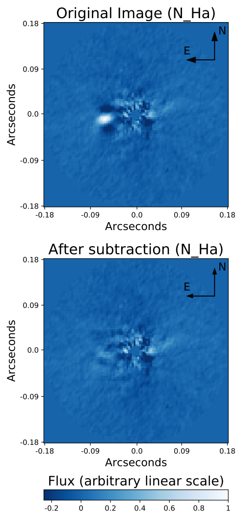
Fig. 3. Image of HD142527 before (top panel) and after (bottom panel) the insertion of the negative companion resulting from the Hessian matrix algorithm. The image flux scale is in both images the same. In this case 14 PCs were subtracted and a mask of 10.8 mas (radius) was applied on the 101 \times 101 pixels images of the N_Ha stack.
