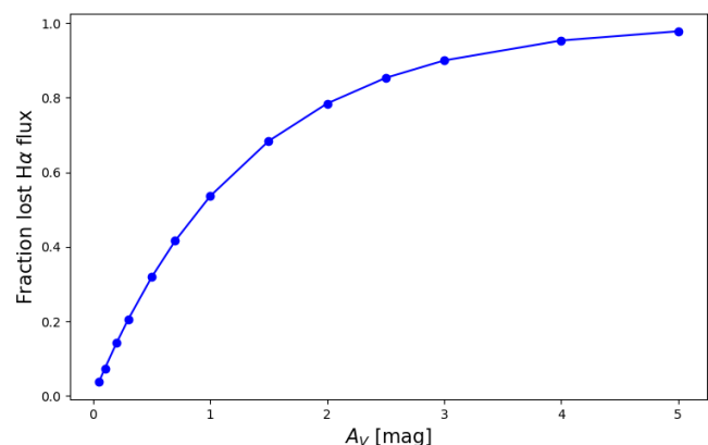
Fig. 11. Fraction of H \alpha flux absorbed as a function of the disk extinction A_V assuming the extinction law of Mathis (1990) as explained in Section 4.1.4.
