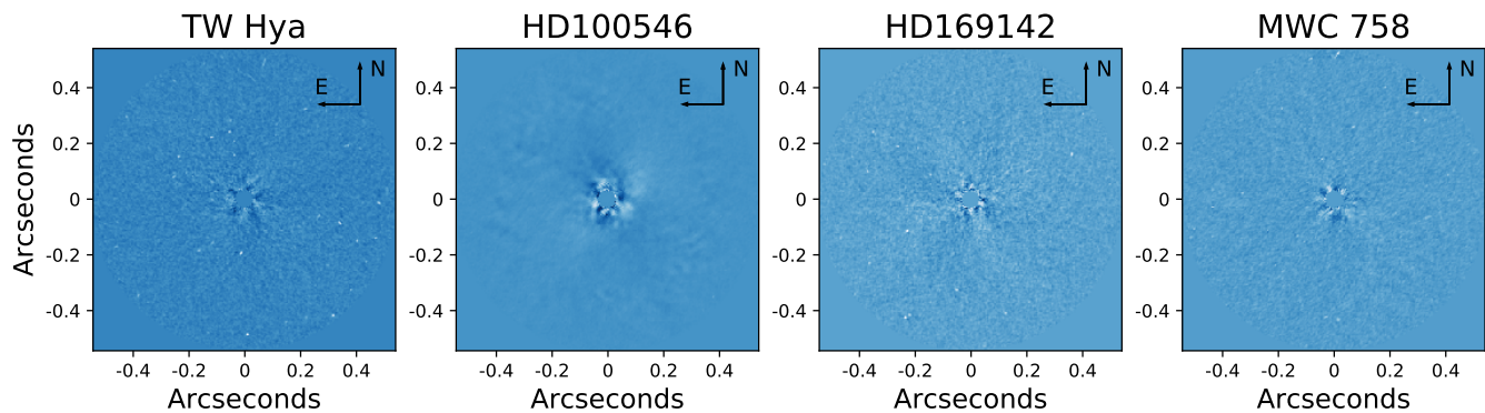
Fig. 6. Final PSF subtracted ADI images of TW Hya, HD100546, HD169142 and MWC 758. We applied a central mask with radius 32.4 mas and 18 PCs were removed. No companion candidates were detected. All images have a linear, but slightly different, color scale.
