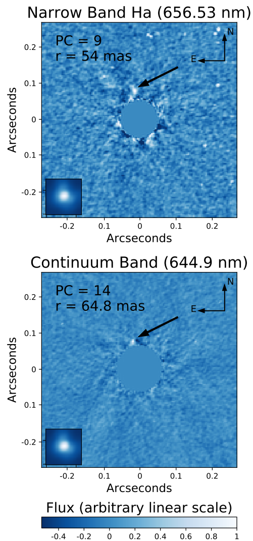
Fig. D.1. Lowest FPF images of HD135344 B (top panel: N_Ha filter; bottom panel: Cnt_Ha filter). The radius r of the inner mask and the number of subtracted PCs are given in each panel. The location of the tentative companion candidate is indicated by the arrow (see Section 4.2.1.).
