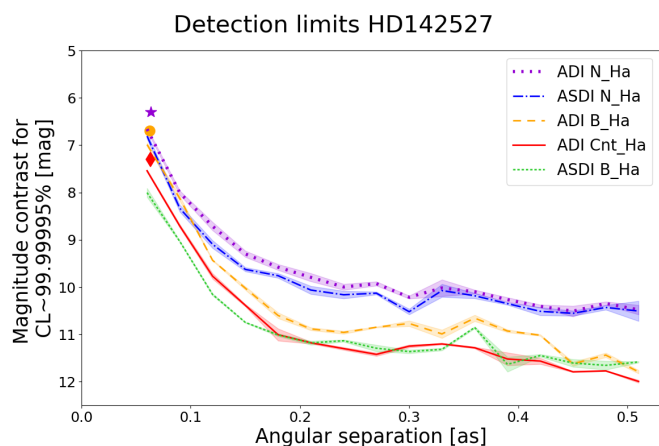
Fig. 2. Contrast curves for HD142527. The colored shaded regions around each curve represent the standard deviation of the achieved contrast at the 6 azimuthal positions considered at each separation. The markers (red diamond, orange circle and violet star) represent the contrast of HD142527 B.
