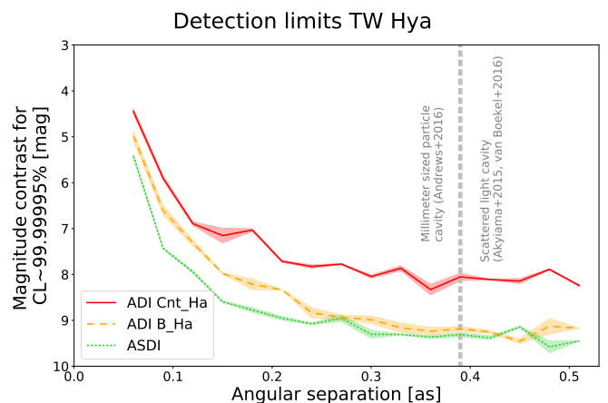
Fig. 7. Contrast curves for TW Hya. The vertical line indicates the gap at 0 ^{\circ} 39 detected in both scattered light (Akiyama et al. 2015; van Boekel et al. 2017) and sub-mm continuum (Andrews et al. 2016).
