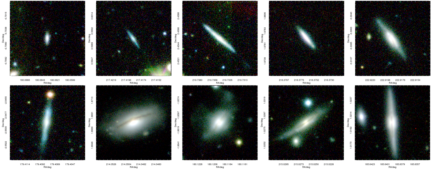
Figure 6. Randomly selected examples with f_{edgeon} > 0.5 from the Galaxy Zoo GAMA sample in order of dust lane vote fraction. Starting at the top left with f_{dustlane} = 0 and ending with f_{dustlane} = 0.9 bottom right.
