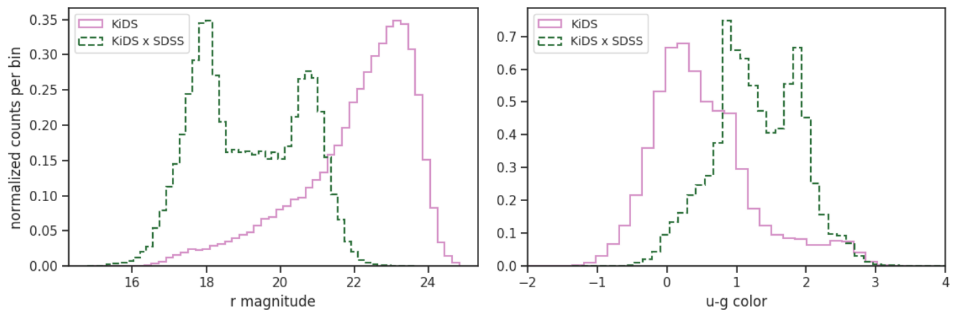
Fig. 1. Normalized histograms of the r -band magnitude (left) and the u - g color (right) for the KiDS inference dataset (pink solid) and the KiDS \times SDSS training set (green dashed), both before applying the r < 22 mag cut. The bimodality of the matched sample is related to SDSS spectroscopic target preselections, preserved by the cross-match with the much deeper KiDS.
