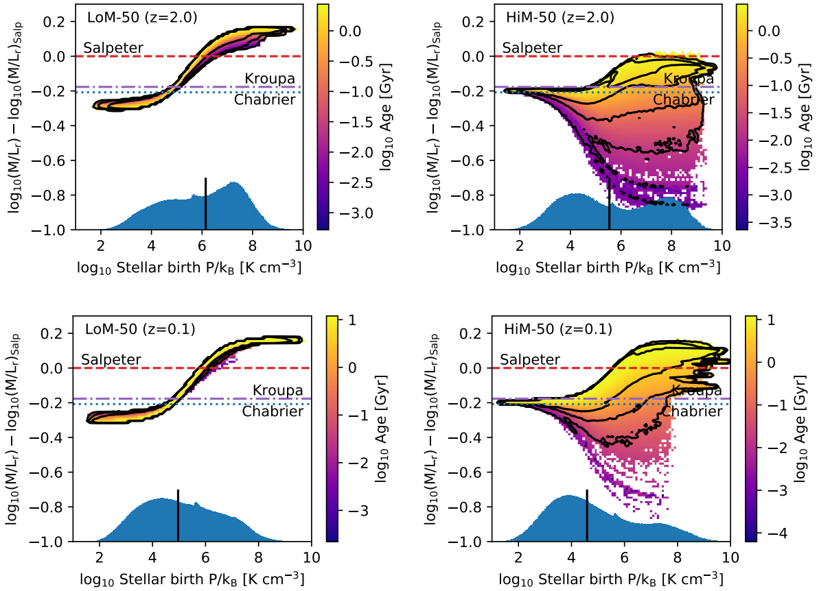
Figure 11. Redshift dependence of the \text{MLE}_{r,\text{Salp}} - \sigma_e relation for individual stellar particles in the LoM-50 (left column) and HiM-50 (right column) simulations. 2D histograms in the upper and lower rows show \text{MLE}_{r,\text{Salp}} as a function of birth ISM pressure for stars within the half-light radius of galaxies with \sigma_e > 100 \text{ km s}^{-1} at z = 2 and z = 0.1 , respectively. 2D bins are coloured by the mean age of stars within each bin. Contours show boundaries of (1000, 100, 10) stars per bin. Blue 1D histograms show the normalized distribution of birth ISM pressures on a linear scale; black horizontal lines show the medians of these distributions. In the LoM-50 case, higher birth ISM pressures at high z result in a larger fraction of dwarf stars than at z = 0.1 . As \text{MLE}_{r,\text{Salp}} is relatively independent of age for this IMF, the effect is immediate. In the HiM case, most stars born at high pressure have not lived long enough for the \text{MLE}_{r,\text{Salp}} to become “heavy” (i.e. for massive stars to die off, reducing the light and increasing the mass due to BHs/NSs), so they still have low M/L ratios relative to Salpeter at this high redshift.
