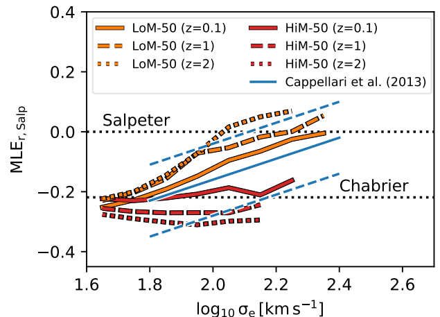
Figure 10. Galaxy-wide \text{MLE}_{r,\text{Salp}} as a function of \sigma_e for LoM-50 (orange) and HiM-50 (red) at z = 0.1 (solid lines), z = 1 (dashed lines), and z = 2 (dotted lines) for all galaxies with \sigma_e > 10^{1.6} \text{ km s}^{-1} at each redshift. Thick lines shown medians for bins with more than 5 galaxies. All quantities are r -band light-weighted and measured within the 2D projected r -band half-light radius of each galaxy. A blue solid line indicates the Cappellari et al. (2013b) relation at z \approx 0 , with dashed blue lines denoting intrinsic scatter. Horizontal black dotted lines mark the Salpeter and Chabrier \text{MLE}_{r,\text{Salp}} values. For the LoM-50 (HiM-50) run, galaxies have a heavier (lighter) \text{MLE}_{r,\text{Salp}} with increasing redshift.
