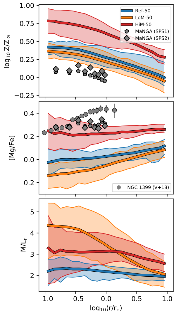
Figure 8. As Fig. 5 but showing, from top to bottom, radial gradients in the stellar metallicity, stellar \alpha -enhancement [\text{Mg}/\text{Fe}] , and r -band stellar M/L ratio for our Sigma150 ETGs. We show metallicity and [\text{Mg}/\text{Fe}] gradients for high-mass galaxies from SDSSIV-MaNGA from Parikh et al. (2018), where pentagons and diamonds correspond to using two different SPS models. The [\text{Mg}/\text{Fe}] radial gradient in NGC 1399 is shown as grey circles (Vaughan et al. 2018b). While negative metallicity gradients are preserved in all of our simulations, the [\text{Mg}/\text{Fe}] gradients are more positive and nearly flat for LoM-50 and HiM-50, respectively. M/L gradients are negative in LoM-50, while in HiM-50 the gradients are much more diverse within r_e .
