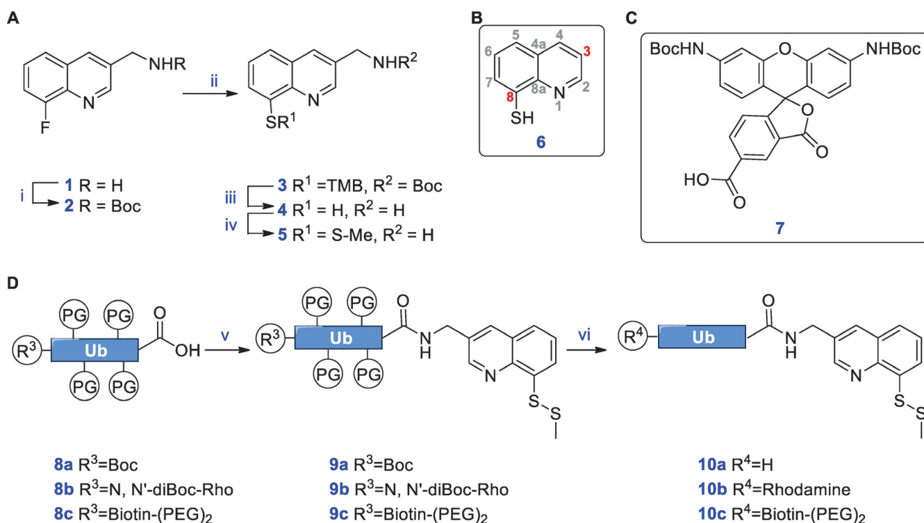
Scheme 1. A) i) Di-tert-butyl dicarbonate, DIPEA, \text{CH}_3\text{CN} , room temperature; ii) TMB-thiol, NaH, THF, 60^\circ\text{C} ; iii) TFA, TES, \text{H}_2\text{O} ; iv) MMTS, MeOH. B) Chemical structure of 8-quinoliniumthiolate ( 6 ) and its carbon positions are indicated. C) N,N' -diBoc-protected rhodamine ( 7 ) used in Fmoc-SPPS of rhodamine-labeled Ub derivatives. D) v) 5 , HBTU, HOBT, DIPEA, room temperature; vi) TFA, TIPS, phenol, \text{H}_2\text{O} . DIPEA = diisopropylethylamine, HBTU = O -(benzotriazol-1-yl)- N,N,N',N' -tetramethyluronium hexafluorophosphate, HOBT = 1-hydroxybenzotriazole, MMTS = S -methyl methanethiosulfonate, PG = protecting group, TES = triethylsilyl, TFA = trifluoroacetic acid, THF = tetrahydrofuran, TIPS = triisopropylsilyl.
