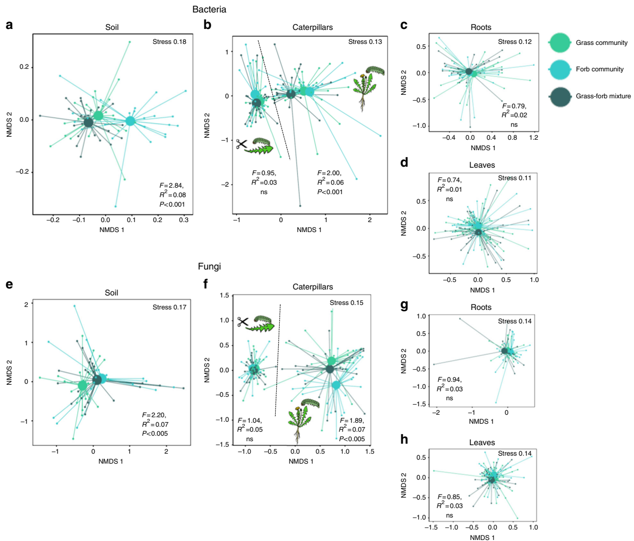
Fig. 3 Legacy effects of plant communities on microbiomes. Plant community identity effects on bacterial a–d and fungal (e–h) communities in caterpillars, leaves, roots, and soil. NMDS plots are presented based on Bray–Curtis similarity. The 2D stress value for each panel ranges between 0.11–0.18. Soils originating from grass communities are presented with light green symbols, soils from forb communities with turquoise symbols and soils from mixed grass and forb communities with dark green symbols. In each panel, smaller symbols depict individual samples, centroids are depicted with larger markers. Significance of the plant community treatment effect based on a PERMANOVA is also presented in each panel. a, e represent the composition of microbiomes in soils, b, f microbiomes in caterpillars both on intact plants and on detached leaves. c, g microbiomes in roots and d, h microbiomes in leaves. The effect of plant community growth rate (fast- and slow-growing communities) is shown in Supplementary Fig. 14
