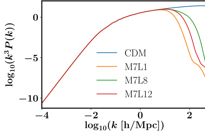
Figure 5.2: Matter Power Spectrum in CDM and various sterile neutrino WDM cosmologies. Sterile neutrinos with mass of m_{SN} = 7 keV and lepton asymmetry numbers L_6 = 1, 8, 12 are shown.
