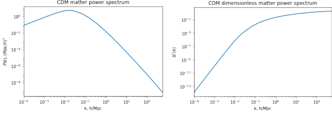
Figure 5.1: CDM Matter Power Spectrum P(k) and dimensionless Matter Power Spectrum \Delta^2(k)
