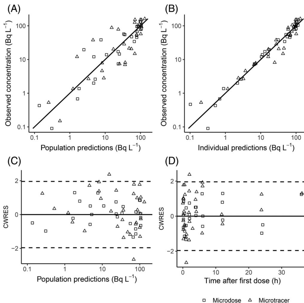
FIGURE 4 Diagnostic plots for [^{14}\text{C}] midazolam pharmacokinetic model, using different symbols for the different treatments. (A) Observed vs population predicted [^{14}\text{C}] midazolam concentrations. (B) Observed vs individually predicted [^{14}\text{C}] midazolam concentrations. (C) Weighted residuals vs population predicted [^{14}\text{C}] midazolam concentration. (D) Weighted residuals vs time. Solid lines represent the line of unity in A and B, and a value of 0 in C and D. Dotted lines represent \pm 1.96 standard deviation, representing the interval in which 95% of the conditional weighted residual (CWRES) values are expected
