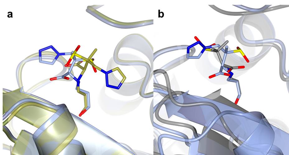
Figure 8. Comparison of the X-ray crystal structures of BlaC and SHV-1 in complex with the trans -enamine adducts of sulbactam and tazobactam. (a) Superposition of wild-type SHV-1 in complex with tazobactam (PDB 1VM1, gold) with Glu166Ala SHV-1 bound to tazobactam (PDB 1RCJ, ice blue). (b) Superposition of BlaC in complex with sulbactam (chain A, gray) with wild-type SHV-1 bound to tazobactam (PDB 1VM1, light blue).
