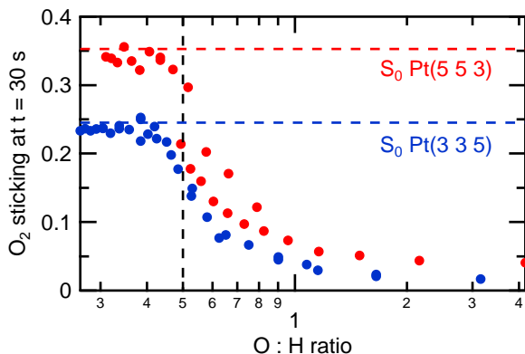
Figure 5.5: O_2 sticking prior to closing the O_2 flag at 240 s as a function of the oxygen:hydrogen ratio (see text) for Pt(3\ 3\ 5) (blue) and Pt(5\ 5\ 3) (red).
