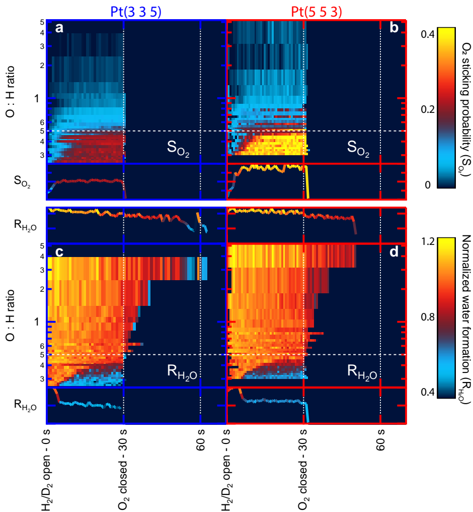
Figure 5.3: Comparison of O 2 sticking (top panels) and normalized water formation (bottom panels), R_{H_2O} , for Pt(3 3 5) (blue axes) and Pt(5 5 3) (red axes) measured as a function of time (bottom axes) and O:H ratio available for reaction at the clean surface (left axes). Normalized water production in panels c and d are extracted from HD formation (see text). At 30 s, the O 2 beam is discontinued. Shown for clarity are the O 2 sticking and R_{H_2O} traces for the lowest O:H ratio and the R_{H_2O} traces for the highest O:H ratio.
