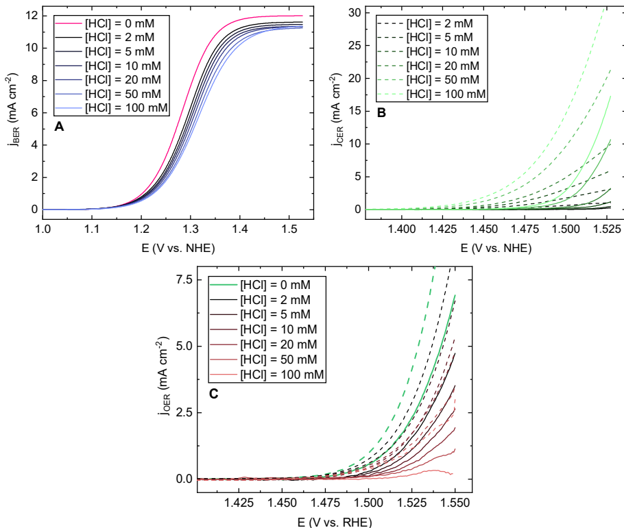
Figure 5.5: Individual BER, CER and OER current densities during parallel \text{Br}^- , \text{Cl}^- and \text{H}_2\text{O} oxidation as function of [\text{HCl}] , on an \text{IrO}_x/\text{GC} electrode in 0.5 \text{ M HClO}_4 and 10 \text{ mM HBr} . A: BER current densities derived from generalized logistic fits of the foot and top of BER waves in Figure 5.1A. Pink trace shows chloride-free conditions. B and C: CER and OER current densities derived from BER logistic fits and the ring response. Solid traces show CER (B) and OER (C) in presence of 10 \text{ mM HBr} . Dashed traces are similar experiments in solutions free of \text{Br}^- . Green, solid trace in C shows OER measured in 0.5 \text{ M HClO}_4 and 10 \text{ mM HBr} only (no \text{Cl}^- ). Green, dashed trace in C shows 'pure OER', measured in 0.5 \text{ M HClO}_4 (no \text{Cl}^- and \text{Br}^- ).
