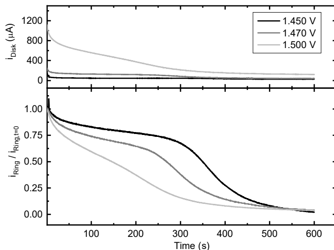
Figure 6.6: Top panel: amperometry measurements at increasing potentials of an \text{IrO}_x/\text{GC} rotating disk electrode (top) in 0.5\text{ M KHSO}_4 , 20\text{ mM KCl} , and 0.6\text{ mM MnSO}_4 ( \text{pH} = 0.87 ), rotation rate 1500\text{ RPM} . The lower panel shows the corresponding i_R normalized to their initial value i_{R,t=0} ( E_R = 0.95\text{ V} ).
