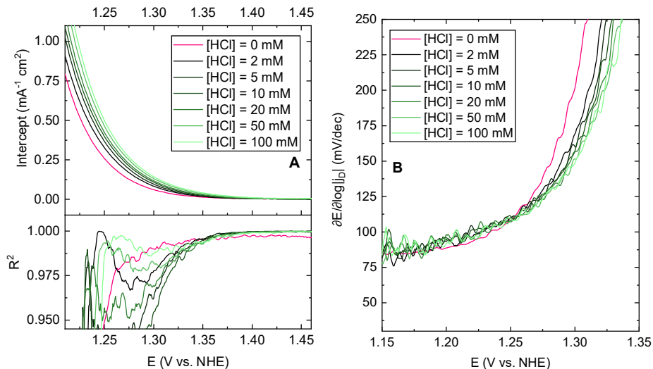
Figure 5.2: Kinetic data measured in the potential region of bromide oxidation, in 0.5 M \text{HClO}_4 + 10 \text{ mM HBr} , for varying concentrations of \text{HCl} . Data is shown on the NHE potential scale to account for minor ( \pm 4 \text{ mV} ) pH shifts. A: Values of the intercept as function of potential, derived from Koutecký-Levich plots as in Figure A 9.5.6. Pink trace shows data when [\text{HCl}] = 0 \text{ mM} . Top panel shows values of the intercept; lower panel shows corresponding values of the linear correlation coefficient R^2 . B: Tafel slopes obtained from semi-logarithmic data of Figure 5.1 (see Figure A 9.5.11).
