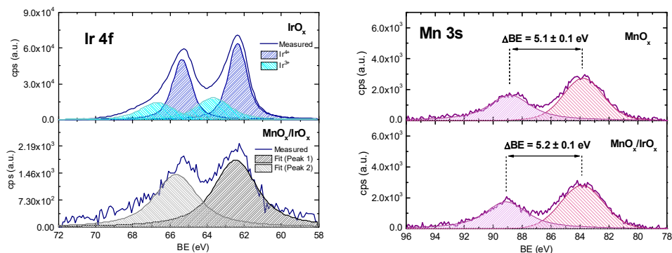
Figure 6.10: Core-level XPS scans of the Ir 4f (left) and Mn 3s (right) spectral peaks, on an absolute intensity scale. Both elements were scanned in samples of their MO x /GC single oxides (top panels) and the mixed MnO x /IrO x /GC sample (lower panels). Note the difference in scale in the lower left-hand panel, illustrating the relatively low intensity of the Ir 4f signal.
