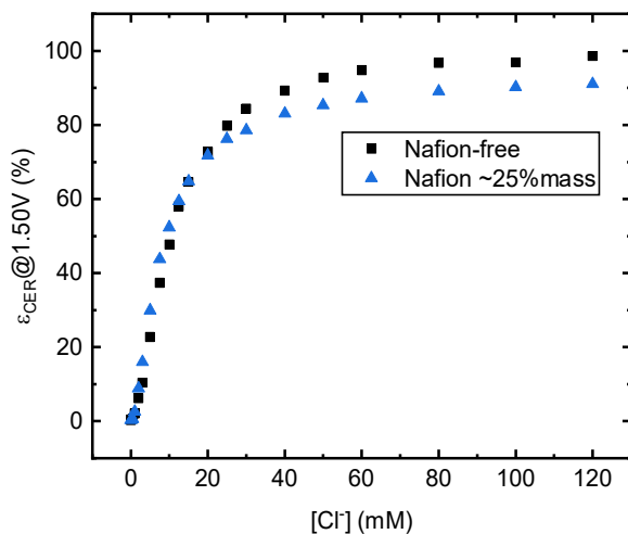
Figure A 9.3.3: The effect of Nafion binder on apparent CER selectivity. Shown is the CER selectivity \varepsilon_{CER} as a function of [Cl^-] in a solution of 0.1 M HClO_4 , for Ba_2PrIrO_6 dropcasted from an EtOH suspension (black) and Ba_2PrIrO_6 dropcasted from an EtOH suspension containing 0.23 mg Nafion copolymer per mg Ba_2PrIrO_6 . Prior to mixing, the Nafion sulfonate groups were partially Na-exchanged by mixing commercial 5%wt stock solution (purchased from Sigma-Aldrich) with 0.1 M NaOH in a ratio of 2:1. Selectivity values shown at 1.50 V, obtained with the RRDE method as described in the main text.
