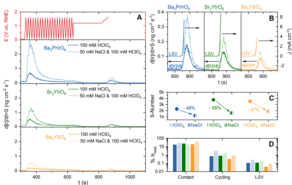
Figure 3.1: Online electrochemical iridium dissolution from ICP-MS measurements. Panel A: Ir dissolution over time correlated with the applied E vs. t protocol (red) for Ba_2PrIrO_6 (blue), Sr_2YIrO_6 (green), and Ba_2YIrO_6 (yellow), in 0.1 M HClO_4 (solid) and 0.1 M HClO_4 with 50 mM NaCl (pale). For clarity reasons, the initial contact peak is not shown (see Figure A 9.3.1 for the full version). Panel B: Ir dissolution along with the current density of the LSV of the E vs. t protocol. Panel C: S-number (amount of gases evolved per amount of Ir dissolved) comparison in presence and absence of 50 mM NaCl. Panel D: Total dissolved amount of Ir during initial contact with the electrolyte, cycling and the LSV, as determined from the initial spot loading (see also Table A 9.3.1).
