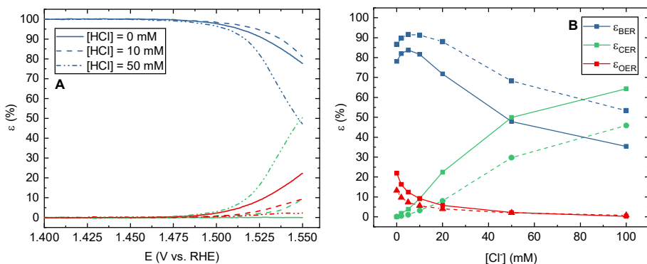
Figure 5.8: Molar selectivities of the BER, CER, and OER in 0.5 M \text{HClO}_4 + 10 mM HBr. A: Data as function of potential, at chloride concentrations of 0 (solid trace), 10 (dashed trace) and 50 mM (dotted trace). Blue, green and red show selectivities for the BER, CER and OER, respectively. B: Data as function of chloride concentration at potentials of 1.535 (dashed trace) and 1.55 V vs. RHE (solid trace). These are potentials where all three reactions are prevalent.
