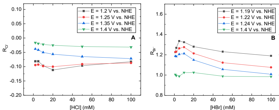
Figure 5.3: Chloride and bromide reaction orders measured in the potential region of bromide oxidation, in 0.5 M \text{HClO}_4 . Data is shown on the NHE potential scale to account for minor ( \pm 4 \text{ mV} ) pH shifts. A: Chloride reaction orders \mathcal{R}_{\text{Cl}^-} at several potentials, obtained by varying the \text{HCl} concentration at a fixed value [\text{HBr}] = 10 \text{ mM} . B: Bromide reaction orders \mathcal{R}_{\text{Br}^-} at several potentials, obtained by varying the \text{HBr} concentration in \text{Cl}^- -free conditions.
