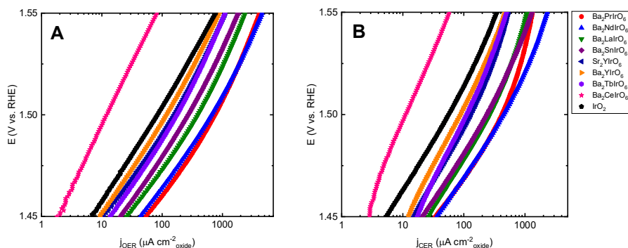
Figure 3.3: OER (A) and CER (B) Tafel curves obtained by scanning the electrode between 1.30 and 1.55 V at 10 mV s -1 . A: ‘pure’ OER current densities in a 0.1 M HClO 4 solution. B: CER current densities in a 0.1 M HClO 4 + 20 mM NaCl solution, derived from ring currents on a Pt ring fixed at 0.95 V vs. RHE. Values shown are the average of at least three independent measurements (see Figure A 9.3.9 for a version containing error bars). Solutions saturated with Ar, rotation rate 1500 RPM.
