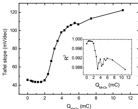
Figure 6.5: Tafel slopes for CER on the disk electrode, constructed from ring currents, as a function of Q_{\text{MnO}_x} . Values taken from CVs similar to Figure 6.2. Inset shows corresponding R^2 values (correlation coefficients), to illustrate the degree of linearity as function of Q_{\text{MnO}_x} .
