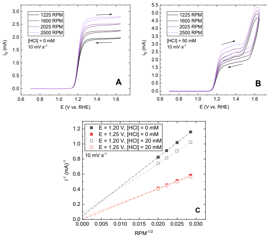
Figure A 9.4.10: Cyclic voltammograms of a Pt-Pt RRDE in a solution of 0.1 M \text{HClO}_4 + 10 mM \text{HBr} . A shows the effect of changing rotation rate, recorded at a scan rate of 10 \text{ mV s}^{-1} . B shows the same experiment in the additional presence of 50 mM \text{HCl} . Arrows indicate scan direction. In C, typical examples of Koutecký-Levich plots are shown obtained from the forward scans of CVs such as shown in A and B.
