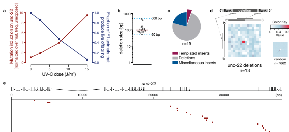
Figure 2. UV-C induced mutagenesis in TLS deficient animals show characteristics of Polθ mediated repair. a) Dose-dependent increased frequency of unc-22 loss of function mutations upon UV-C exposure (in red). Dose dependent decrease in animal fertility (in blue). b) Size representation of UV-induced unc-22 deletion alleles (n=17). c) Distribution of deletion alleles: the majority are simple deletions (in grey), without containing insertions in between both breakpoints. Three alleles have small miscellaneous inserts of 1 to 6 bp (in blue), whereas one allele (in magenta) has an insert that is templated from the flank of the break (see also Suppl. table 2). d) A heat map representation of micro-homology at deletion breakpoints of simple deletion alleles. The bases that flank the right and left deletion breakpoints and are either retained or lost in the deletion alleles are plotted against each other. The heat map, representing 15 simple deletions, reveals overrepresentation of 1 nucleotide of micro-homology. A heat map for a simulated set of random deletions (n=7662) with random distribution is displayed on the right. e) A schematic representation of the unc-22 gene with underneath the position and size of the deletion alleles represented as red bars.
