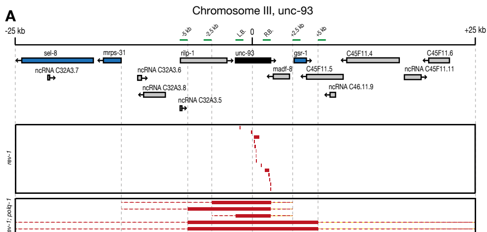
Figure 3. In absence of REV-1 unresolved replication blocks lead to TMEJ substrates.
