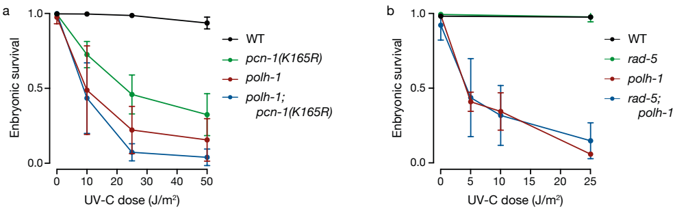
Figure S2. a+b) Hermaphrodite adult animals of indicated genotypes were exposed to different doses of UV-C and the embryonic survival of the progeny, as a fraction of the total brood, was determined for a 20 hours time period post irradiation.
