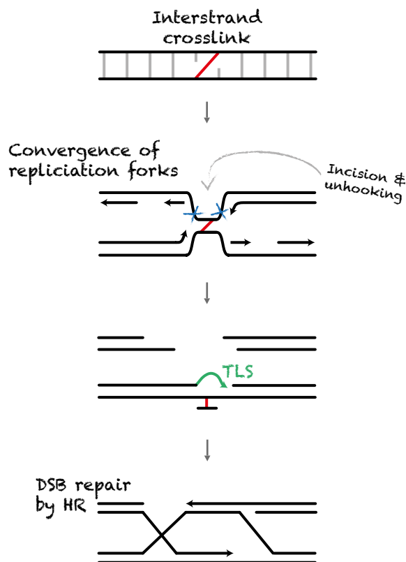
Figure 3. A schematic of interstrand crosslink repair. For details see text.
