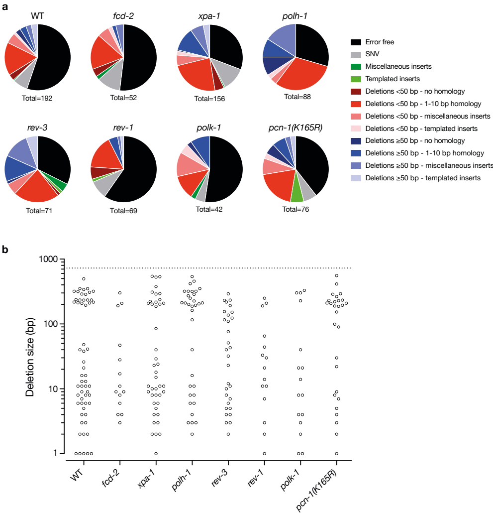
Figure 3. Mutational spectra observed in different DNA response deficient backgrounds. a) All pICL repair products obtained after sequencing are presented for the indicated genotypes. Categories of repair products were based on observations in WT. b) Sizes of unique deletions observed in the indicated genotypes.
