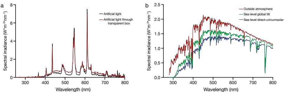
Figure S2. a) Radiospectrogram of the spectral irradiance of the artificial light in our lab. It contains low levels of UV-A and -B with a clear peak at 366 nm and also substantial ammounts of high energy violet end blue light (400-500 nm). b) Radiospectrogram of regular daylight measured in spectral irradiance. Source: ASTM Terrestrial Reference Spectra for Photovoltaic Performance Evaluation ( http://rredc.nrel.gov/solar/spectra/am1.5 ). No data was available for wavelengths lower than 280 nm. However, it is known that UV-C light with wavelengths between 100 and 280 nm is efficiently absorbed by the ozone layer and does not reach the Earth's surface.
